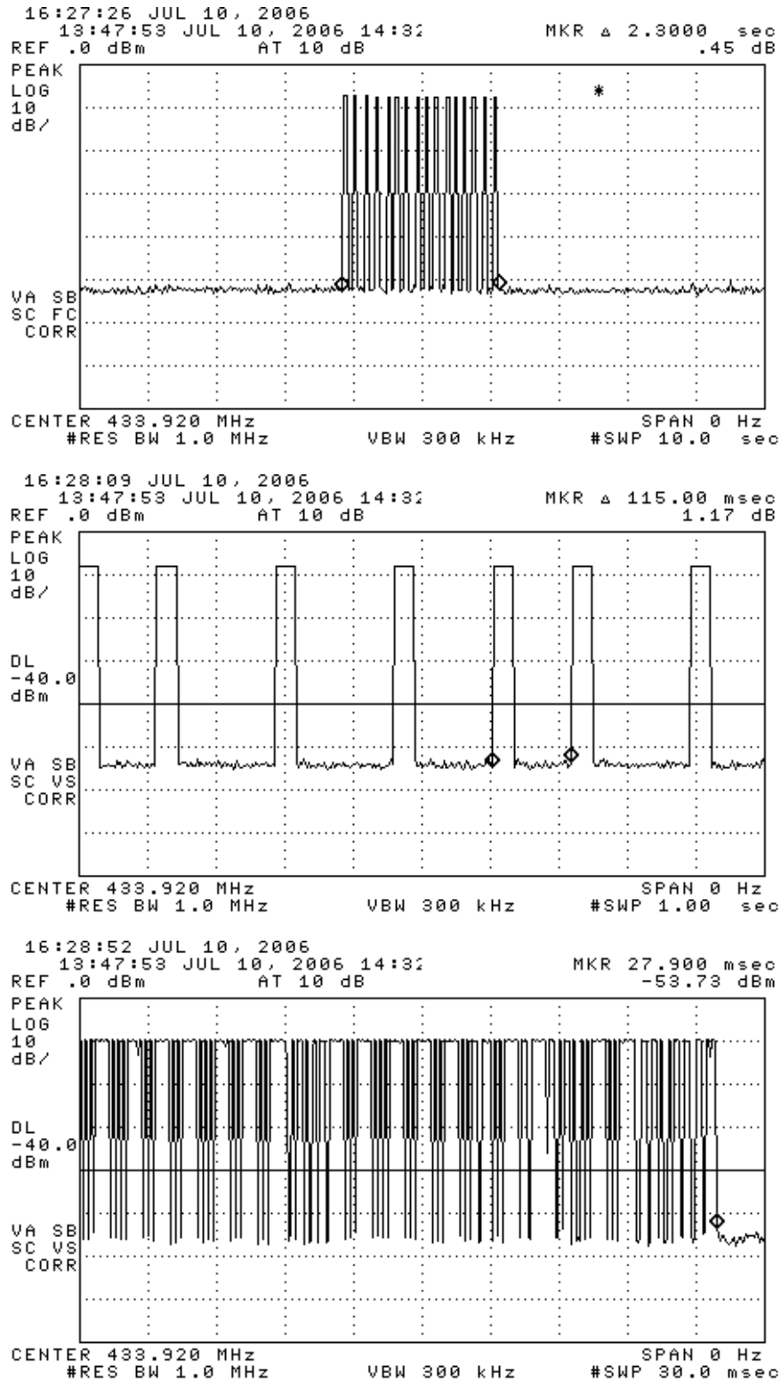
Figure 6.1(a). Transmissions modulation characteristics: (top) LF act. transmission, (center) minimum word separation, (bottom) expanded word.
