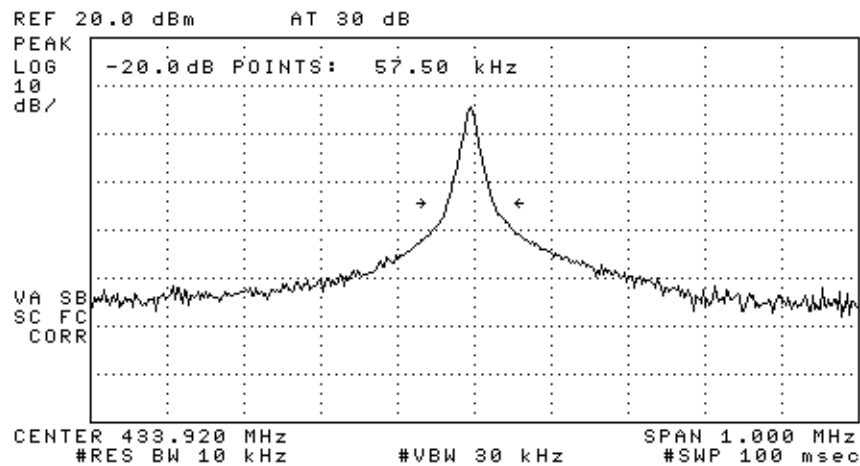
Figure 6: Intentional Emission Bandwidth.
