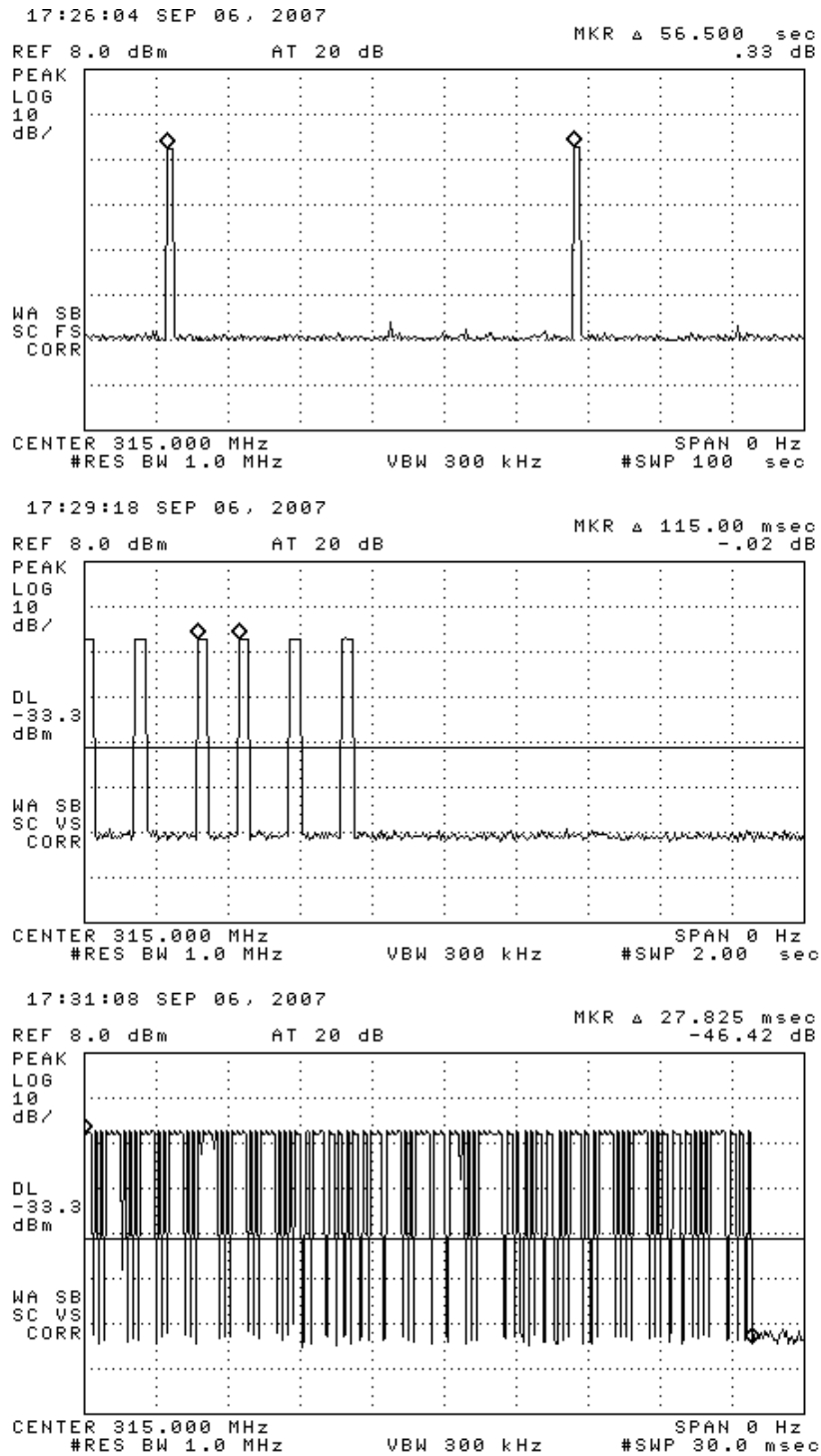
Figure 6.1(a). Transmissions modulation characteristics: (top) regular transmission, (center) 6 packets, (bottom) single packet.
