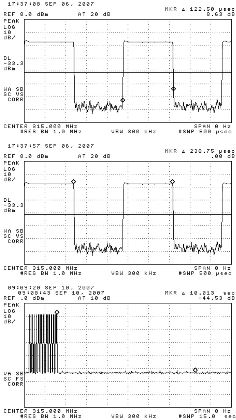
Figure 6.1(b). Transmissions modulation characteristics: (top) Manchester width, (center) Manchester period, (bottom) LF interrogation Turn Off.
