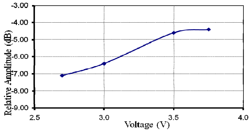
Figure 6.4. Relative emissions at 315 MHz vs. supply voltage (cw emission).
