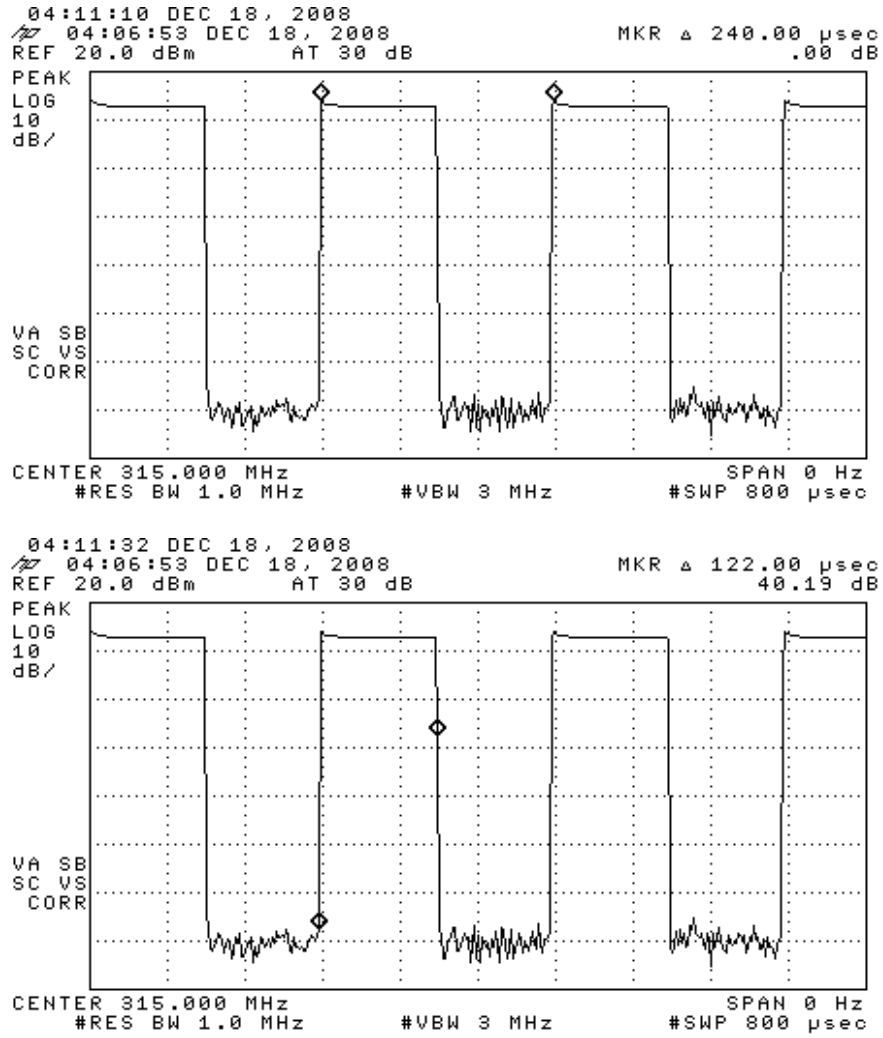
Figure 6.1(b). Modulation characteristics. (top) Manchester period, (bottom) Manchester pulse-width.
