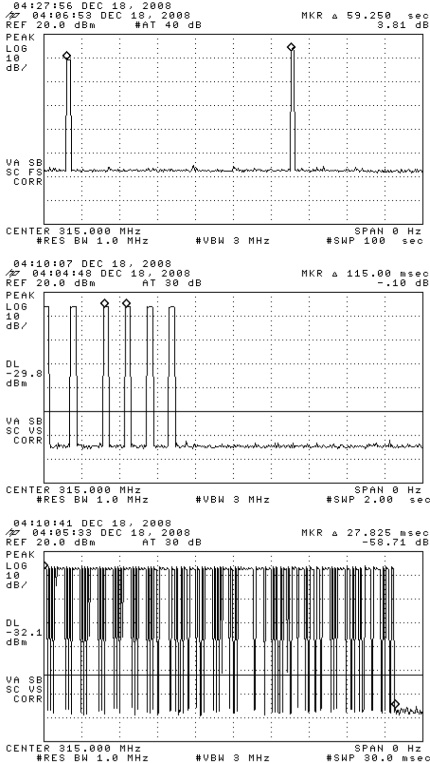
Figure 6.1(a). Transmission modulation characteristics. (top) roll-mode transmission – 6 frames, (center) minimum frame period, (bottom) expanded word.
