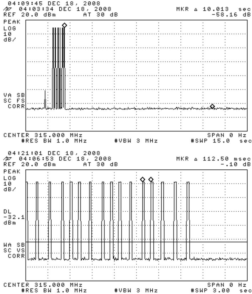
Figure 6.1(c). Transmission modulation characteristics. (top) response to manual LF interrogation – 16 frames, (bottom) minimum word period in transmission.
