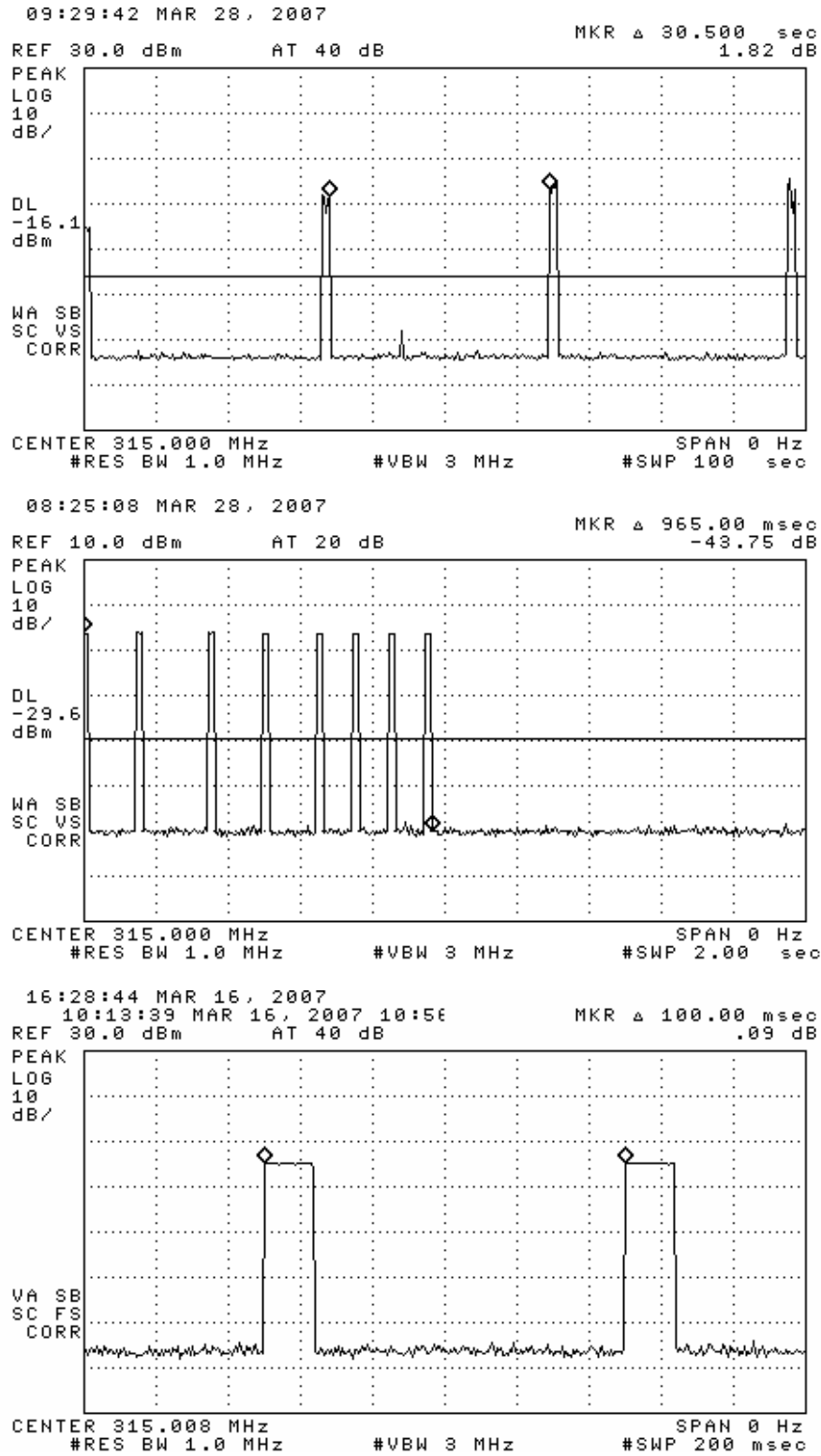
Figure 6.1(a). Transmissions modulation characteristics: (top) factory mode transmission (worst case), (center) expanded dataset, (bottom) expanded word.
