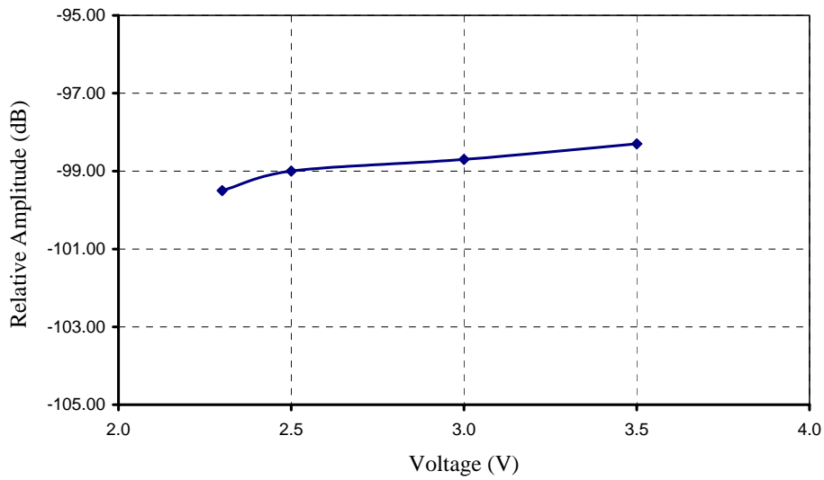
Figure 6.4. Relative emissions at 315.0 MHz vs. supply voltage. (pulsed emission)
