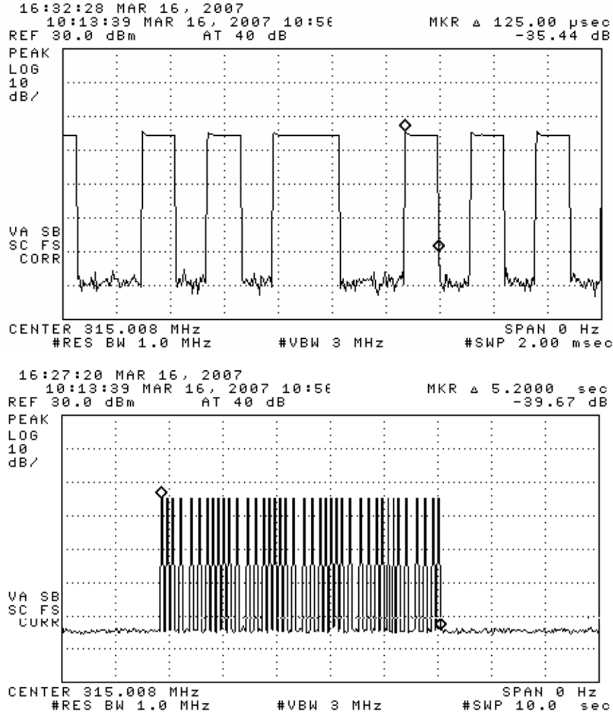
Figure 6.1(c). Transmissions modulation characteristics: (top) Manchester pulse, (bottom) Learn Mode transmission (LF actuated).
