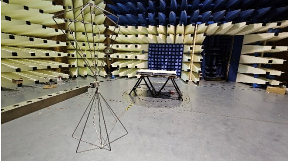
Fig A1: Radiated Emissions 30MHz -300MHz
