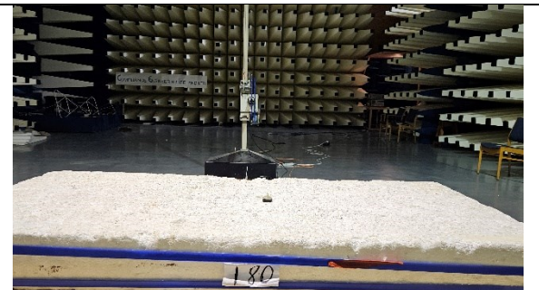
Fig A4: Radiated Emissions 300MHz -1GHz
