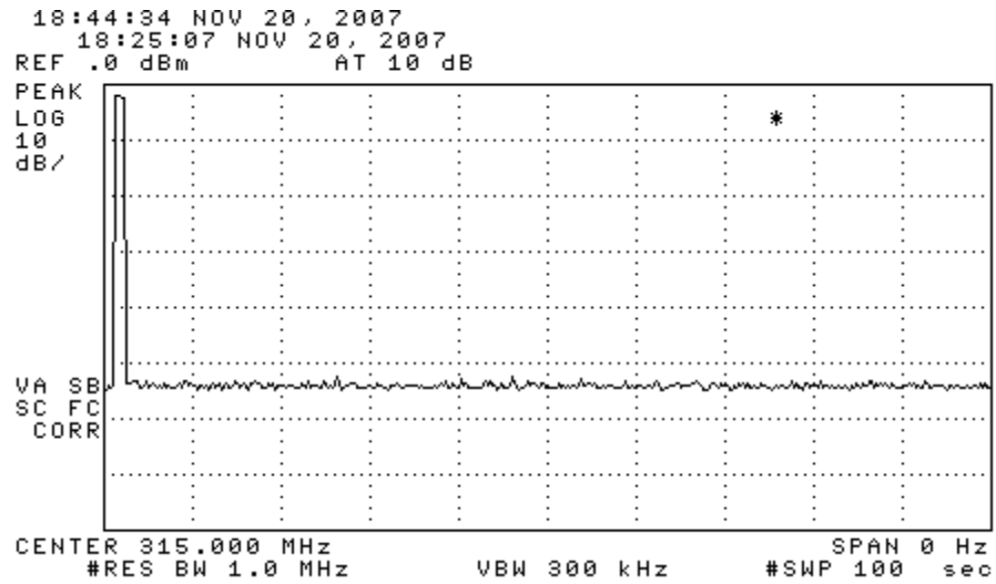
Figure 6.1(d). Stationary Mode (1 Transmission / 6 Hrs).
