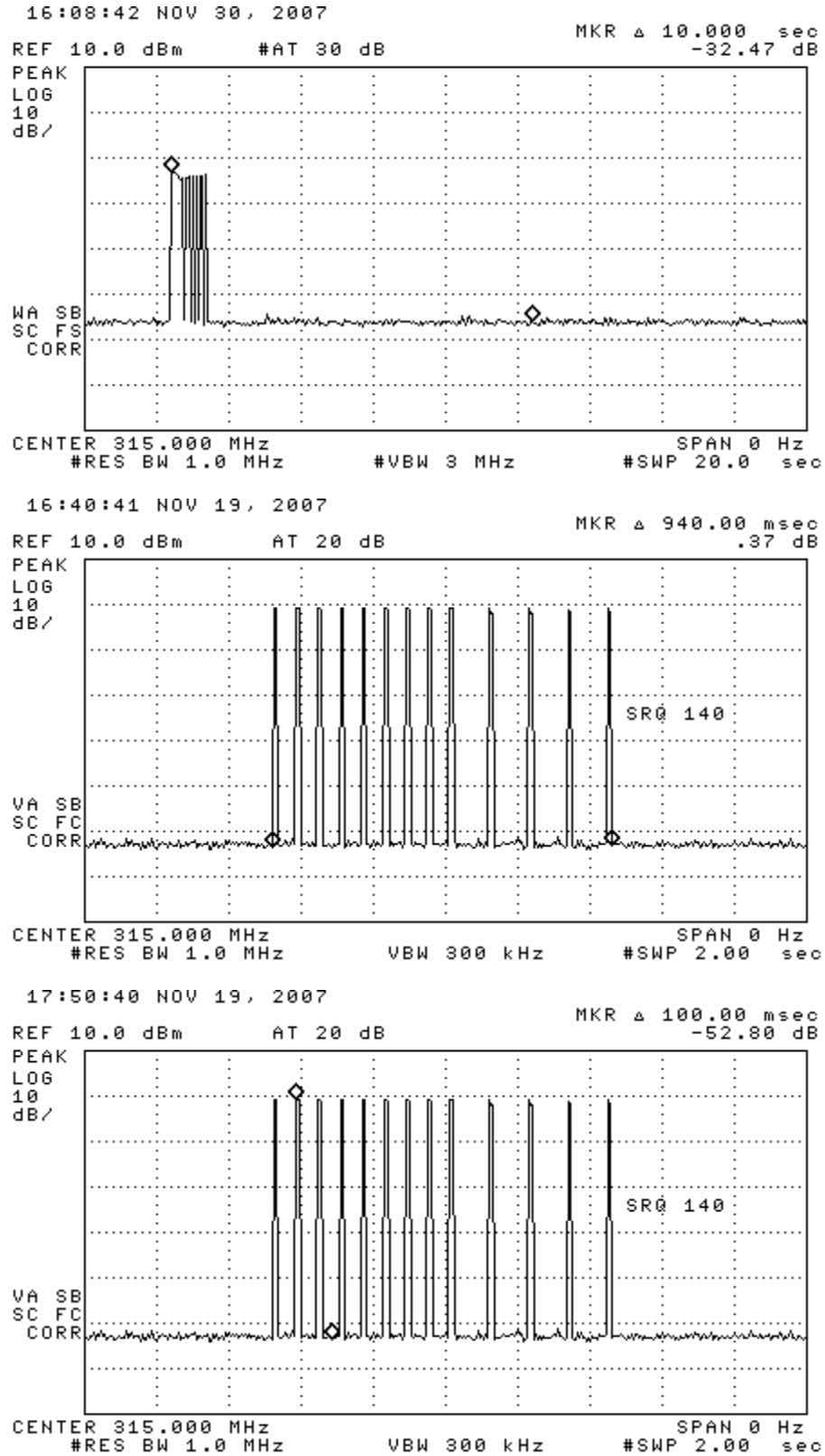
Figure 6.1(b). (top) 9 ASK + 4 FSK single LF service mode interrogation, (center) expanded 9 ASK + 4 FSK transmission, (bottom) two ASK words / 100 ms window.
