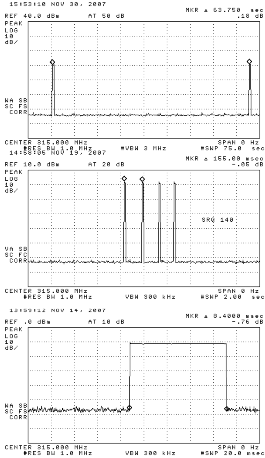
Figure 6.1(a). Transmissions modulation characteristics: (top) FSK (roll mode) transmission, (center) FSK word, (bottom) expanded bit.
