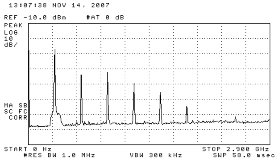
Figure 6.2. Emission spectrum of the DUT (pulsed). The amplitudes are indicative (un-calibrated).
