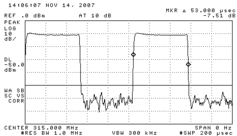
Figure 6.1(c). (top) ASK word, (center) expanded ASK word, (bottom) ASK Manchester encoding.
