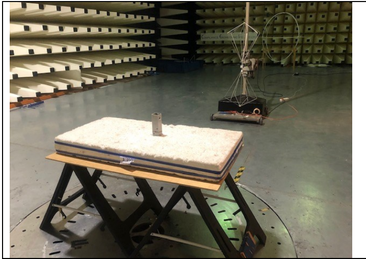
Fig 1a Test setup 30MHz -300MHz Rad Emissions
