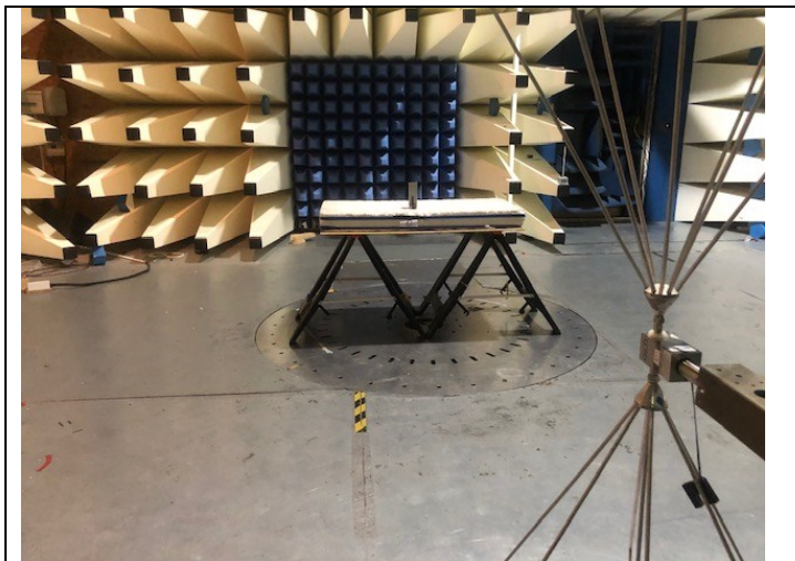
Fig 1b Test setup 30MHz -300MHz Rad Emissions
