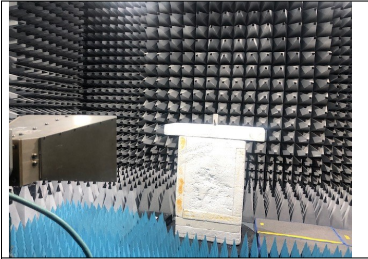
Fig 3 Test setup 1GHz 6GHz Rad Emissions
