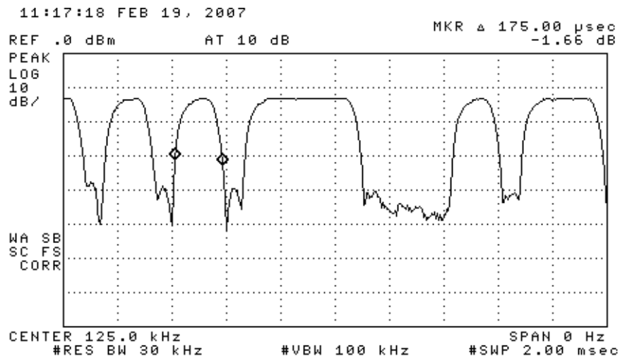
Figure 6.1(a). Transmission modulation characteristics.
