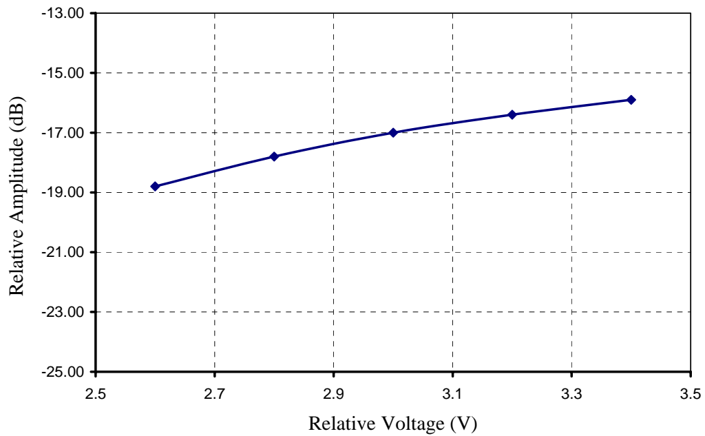
Figure 6.4. Relative emission at 135 kHz vs. supply voltage.
