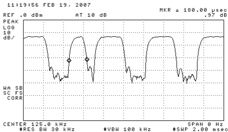
Figure 6.1(b). Transmission modulation characteristics.
