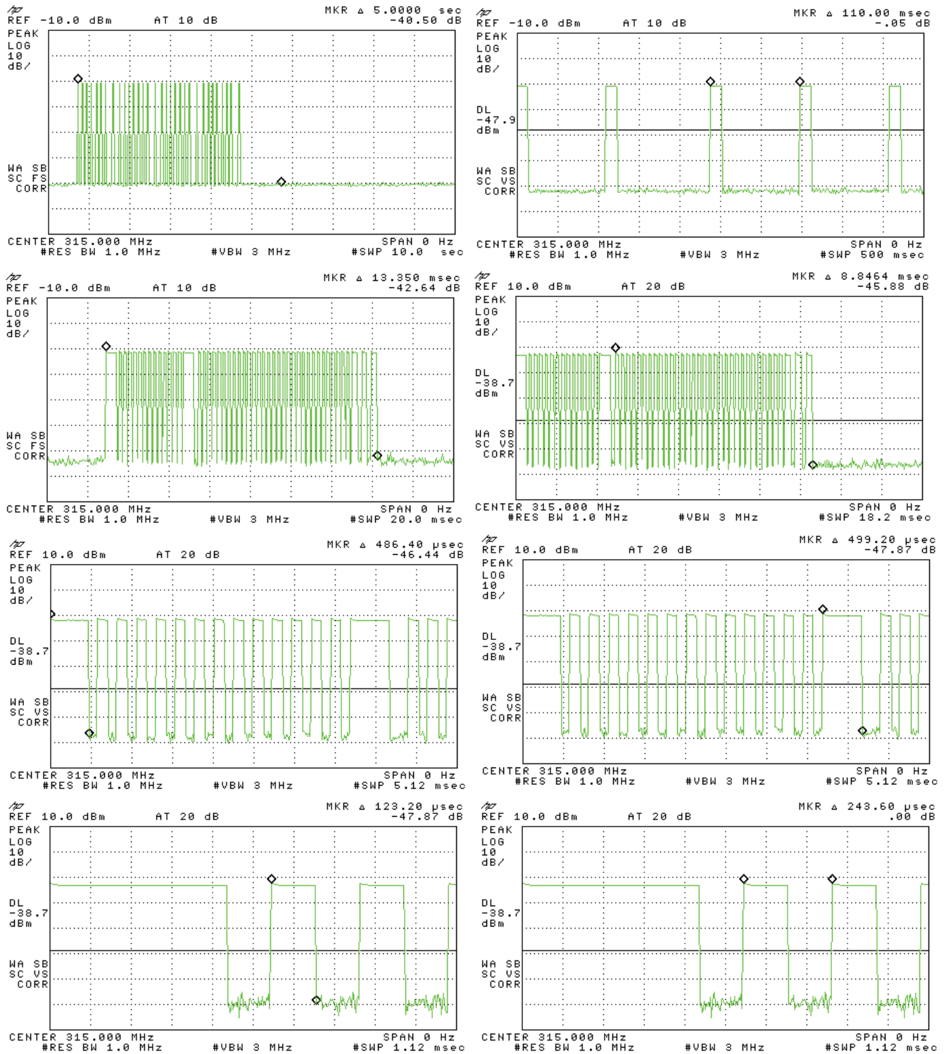
Figure 5(c): Pulsed Emission Characteristics (Duty Cycle).
