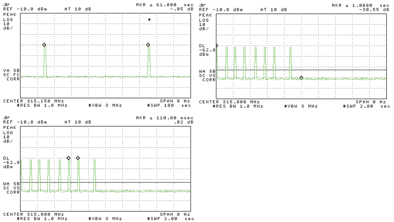
Figure 5(d): Pulsed Emission Characteristics (Duty Cycle).
