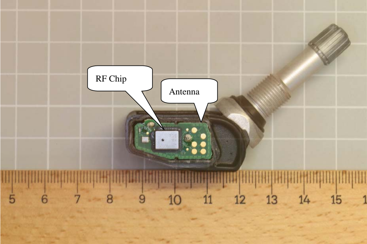
(9) EUT Photo – RF Chip + Antenna
