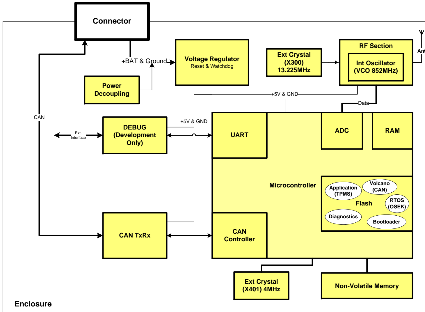
Fig.1 : Chrysler Corax Block Diagram
