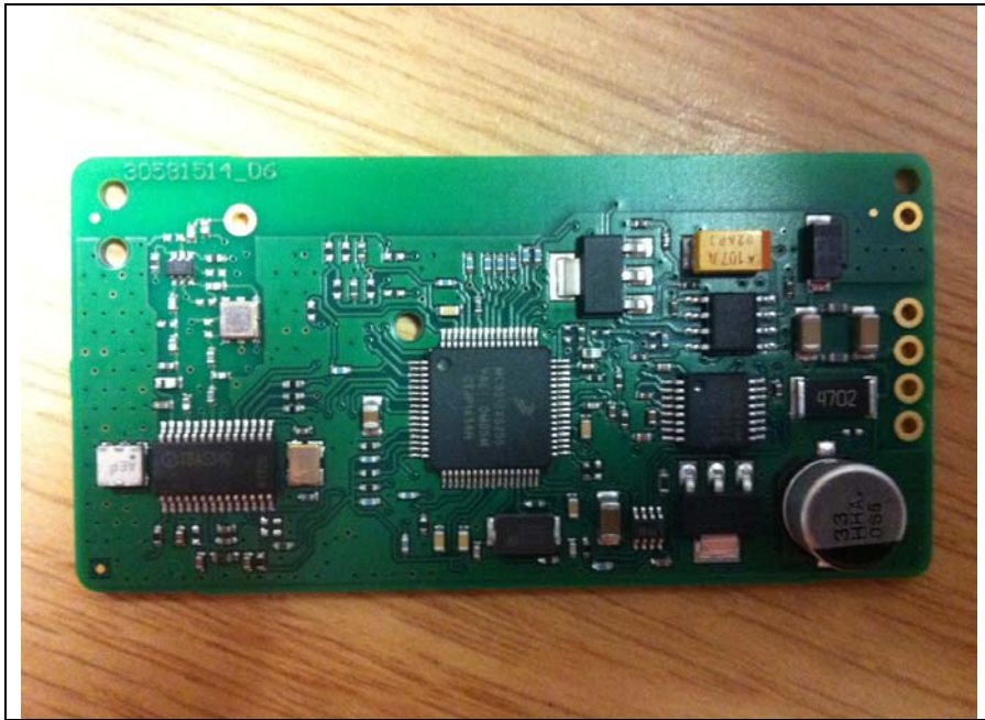
Internal View 1
