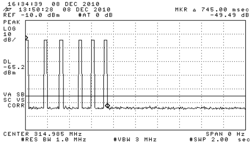
Figure 6.1(b). Worst-case Periodic Transmission. (top) transmission repetition rate, (bottom) transmission length.
