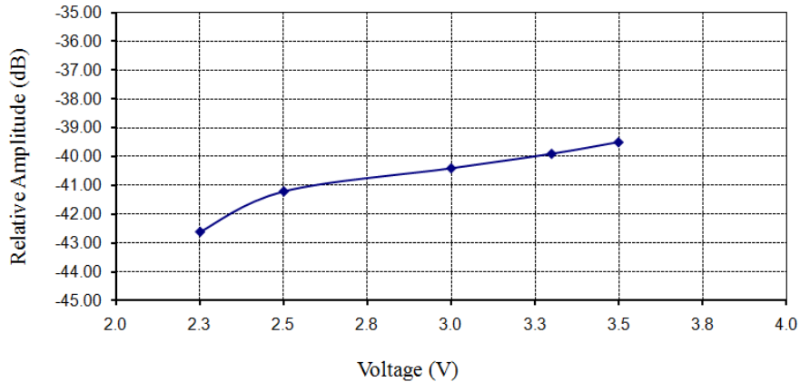
Figure 6.4. Relative emission at fundamental vs. supply voltage (cw).
