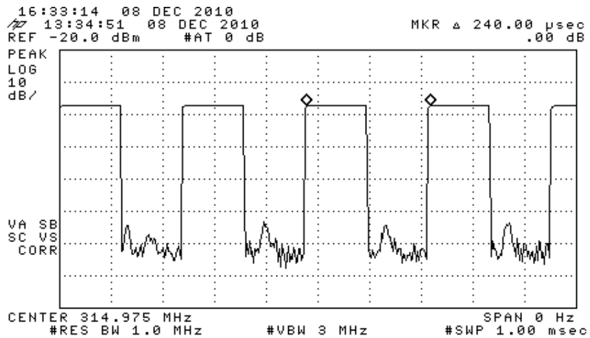
Figure 6.1(c). Frame Encoding. (top) Manchester encoding, (center) Manchester pulse period, (bottom) Manchester pulse width.
