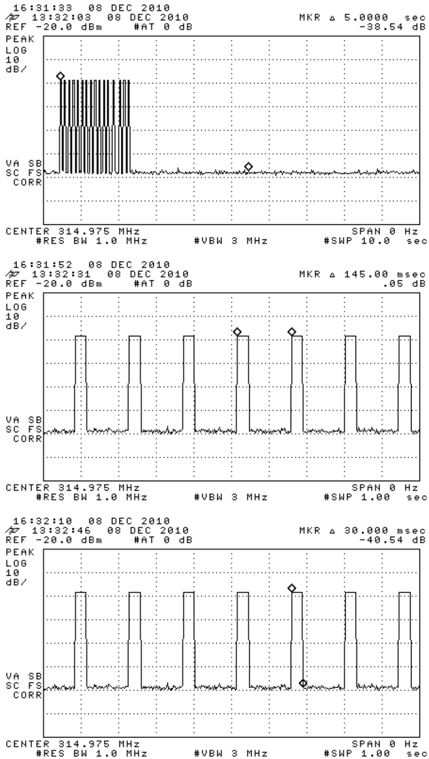
Figure 6.1(a). Manual LF Activated Transmission. (top) complete transmission, (center) expanded frame period, (bottom) frame width.
