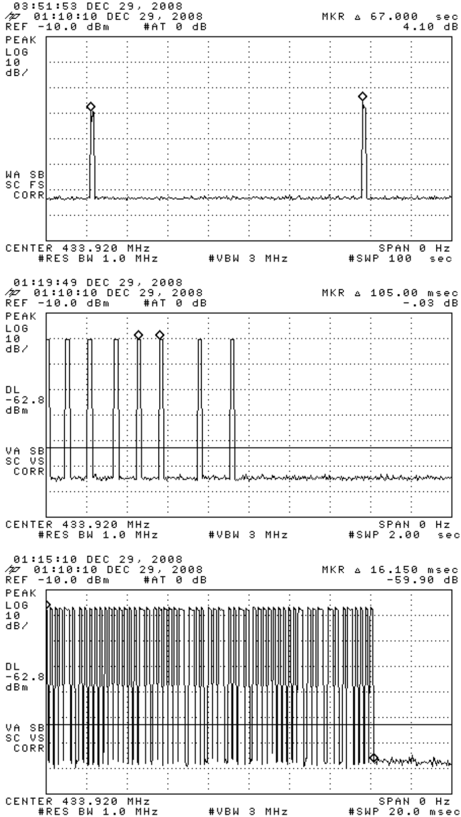
Figure 6.1(a). Transmission modulation characteristics. (top) roll-mode transmissions, (center) expanded transmission, (bottom) expanded word.
