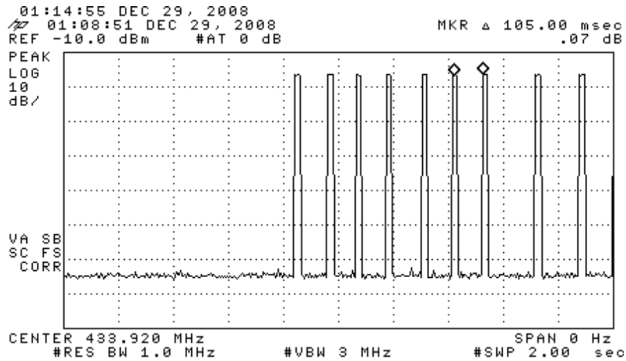
Figure 6.1(c). Transmission modulation characteristics. (top) response to manual LF interrogation, (bottom) minimum word period in transmission
