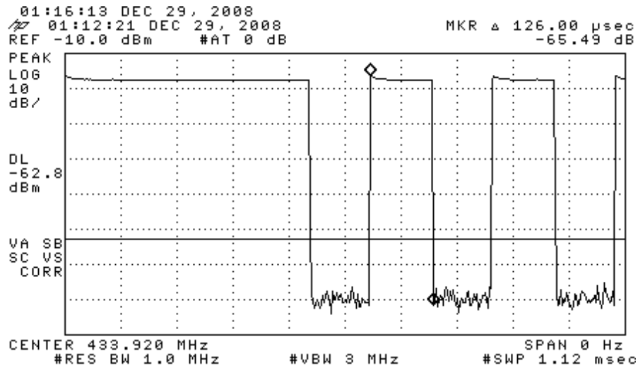
Figure 6.1(b). Transmission modulation characteristics. (top) expanded word, (center) Manchester period, (bottom) Manchester pulse-width.
