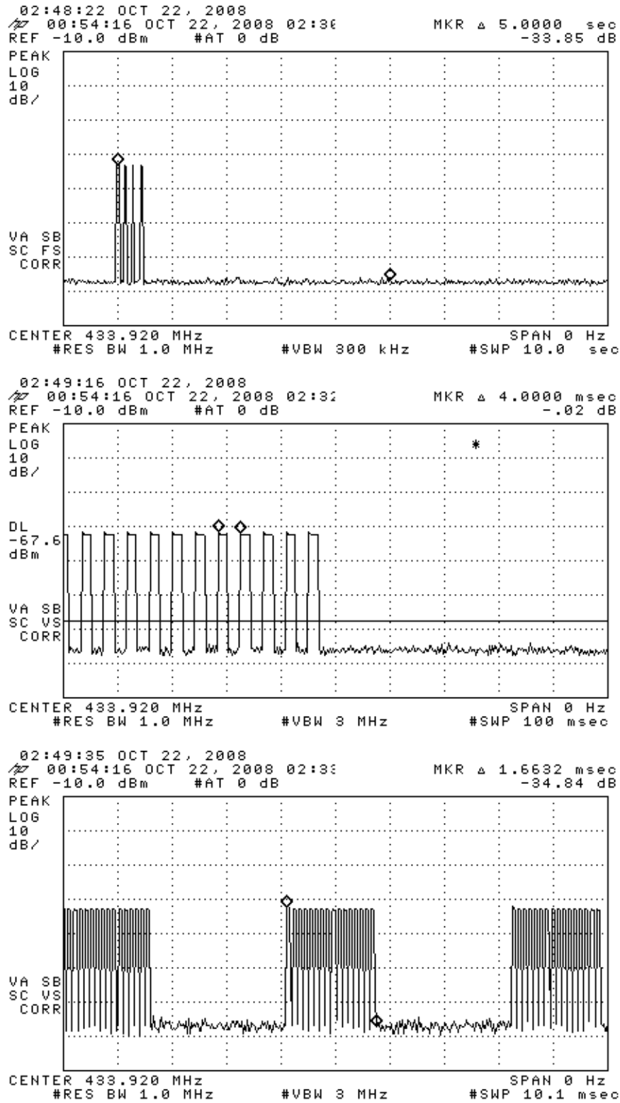
Figure 6.1(a). Transmission modulation characteristics. (top) LF response transmission, (center) expanded worst case LF words, (bottom) expanded word showing Manchester encoding (~50% duty).
