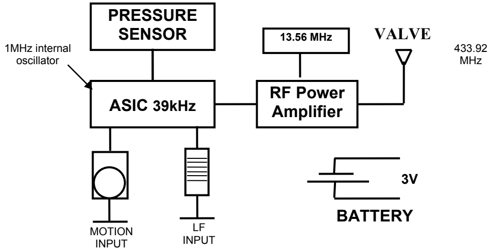
Chrysler Snap In 433.92 MHz Block Diagram
