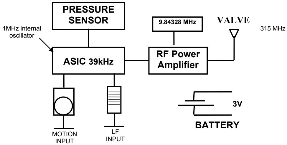
Chrysler Snap In 315 MHz Block Diagram
