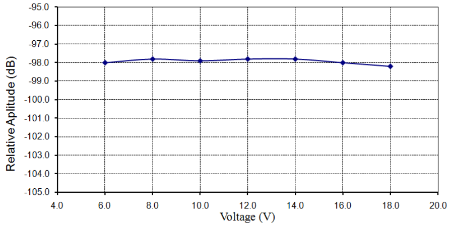
Figure 6.4. Relative emission vs. supply voltage.
