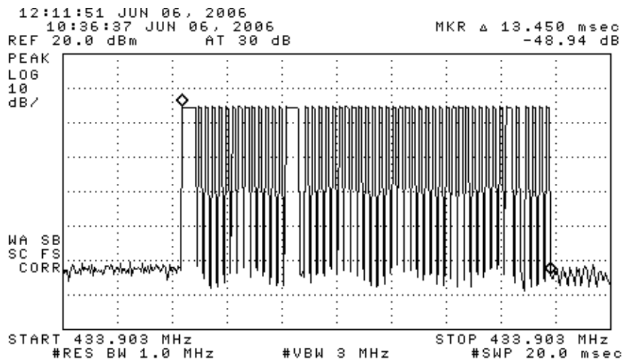
Figure 6.1(a). Transmissions modulation characteristics: (top) complete transmission, (center) expanded period, (bottom) expanded word.
