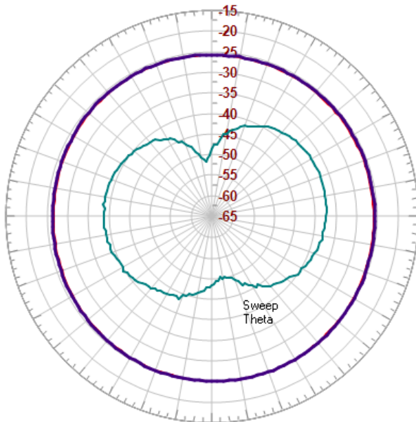
Phi = 0 (dBi)
