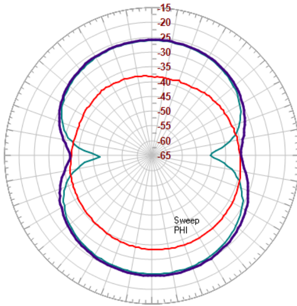
Theta = 0 (dBi)
