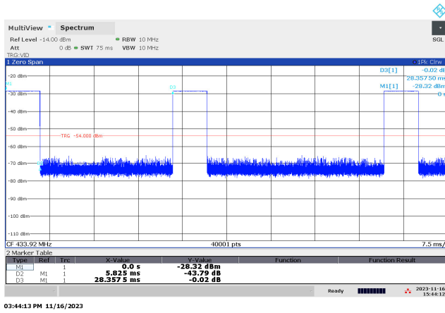
Figure 4.2(iii) Fundamental Emission Pulsed Operation.
