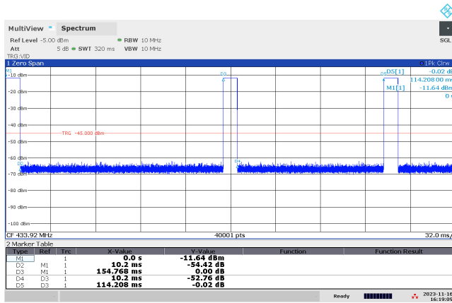
Figure 4.2(iv) Fundamental Emission Pulsed Operation.
