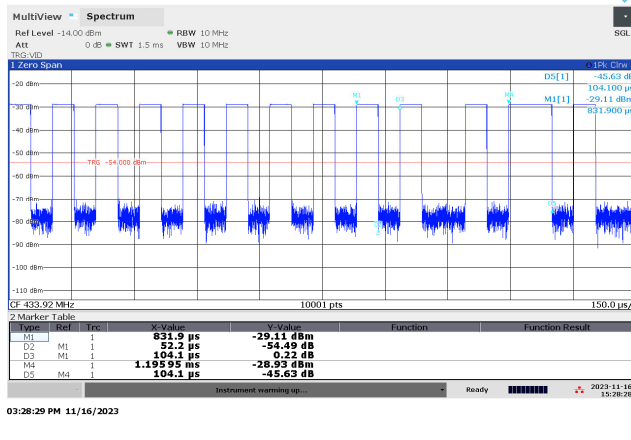
Figure 4.2(i) Fundamental Emission Pulsed Operation.
