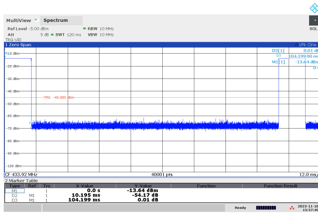
Figure 4.2(ii) Fundamental Emission Pulsed Operation.
