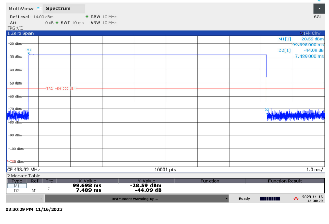
Figure 4.2(i) Fundamental Emission Pulsed Operation.
