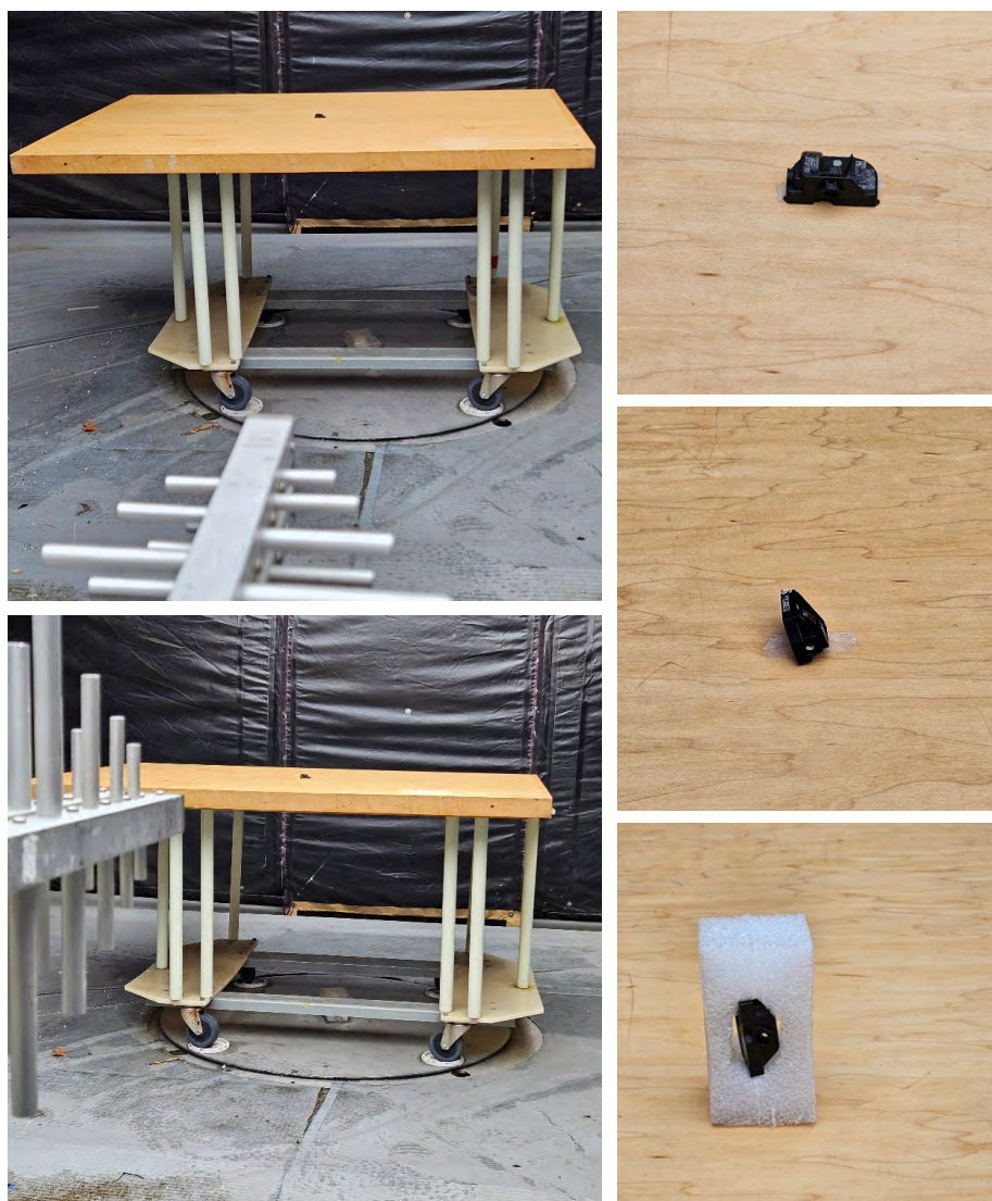
Figure 4.1(i) Radiated Emissions Test Setup Photograph(s).
