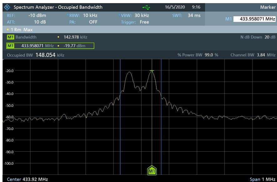
Figure 6: Fundamental Emission Bandwidth.
