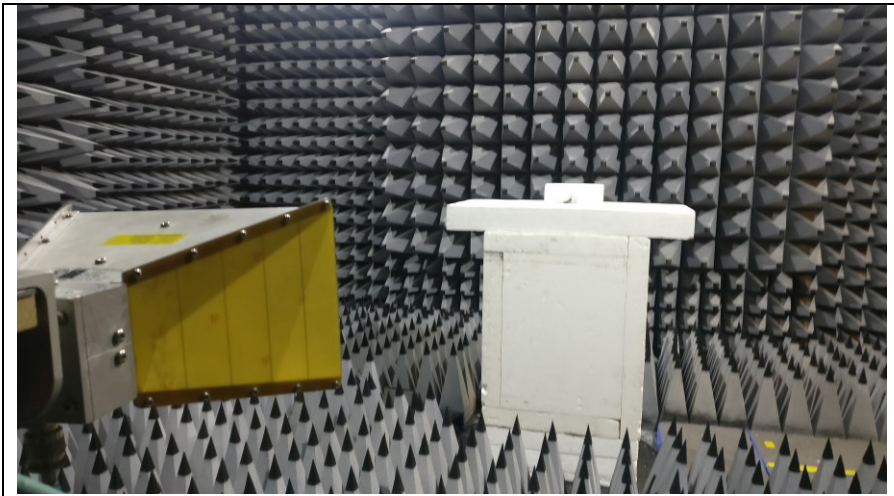
Fig 3 Test setup 1GHz -6GHz Rad Emission
