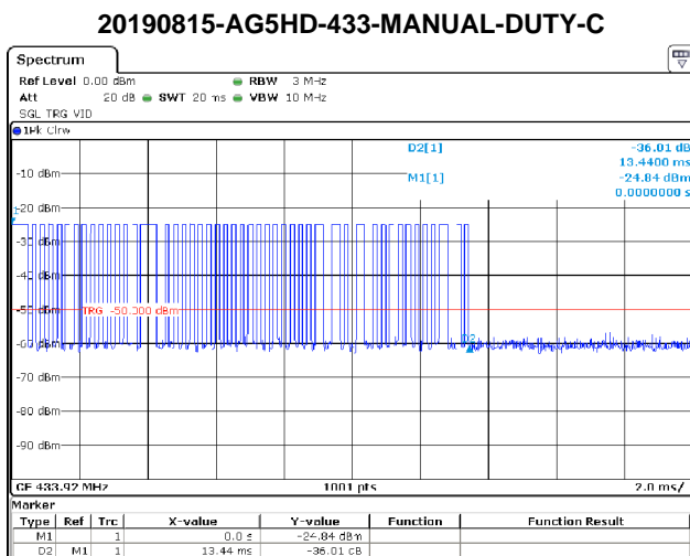
Figure 5(d): Fundamental Emission Pulsed Operation.
