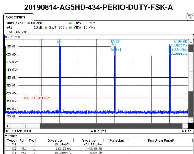
Figure 5(c): Fundamental Emission Pulsed Operation.
