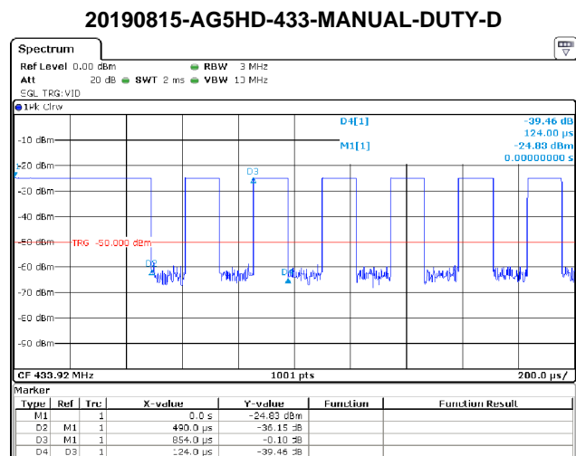
Figure 5(d): Fundamental Emission Pulsed Operation.
