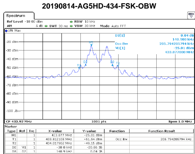
Figure 6: Fundamental Emission Bandwidth.
