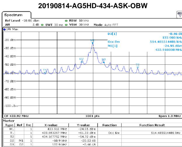
Figure 6: Fundamental Emission Bandwidth.
