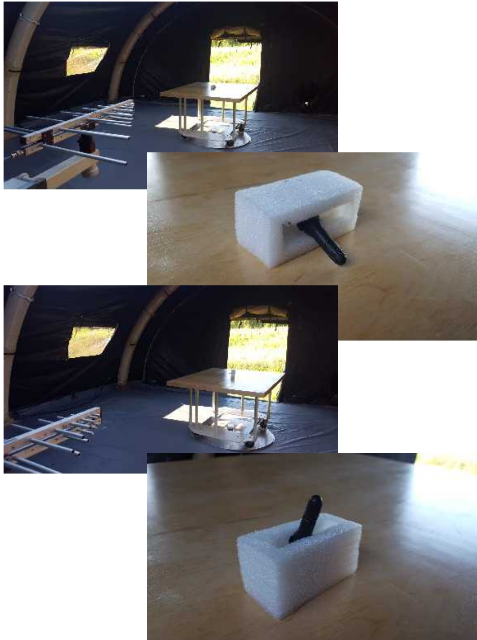
Figure 4: Radiated Emissions Test Setup Photograph(s).
