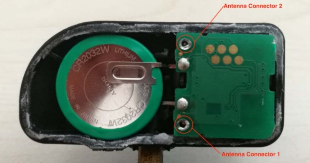
(7) EUT Photo
