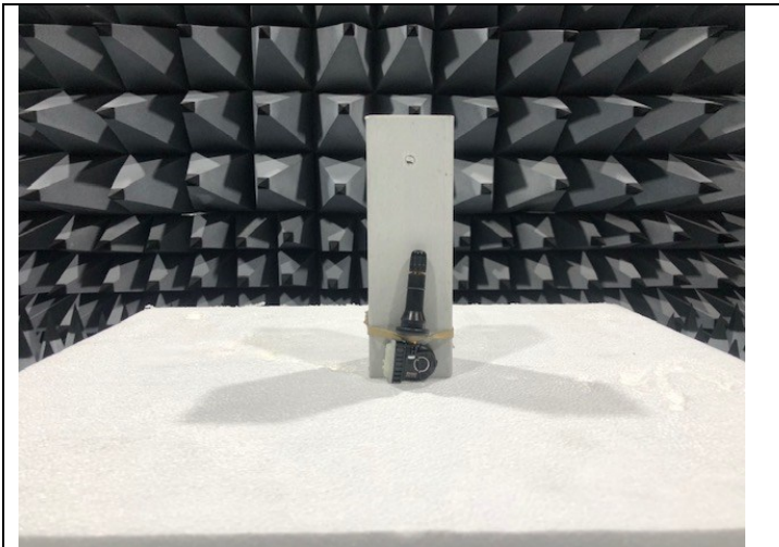
Fig 4a EUT close up Rad Emissions
