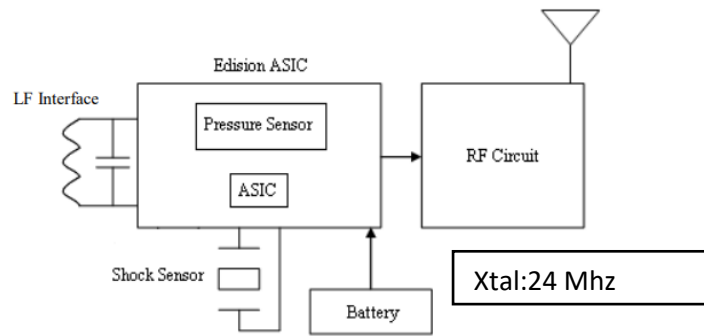
Figure 1 - TPM Sensor Block Diagram
