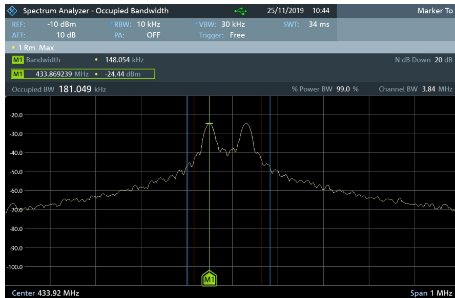
Figure 6: Fundamental Emission Bandwidth.
