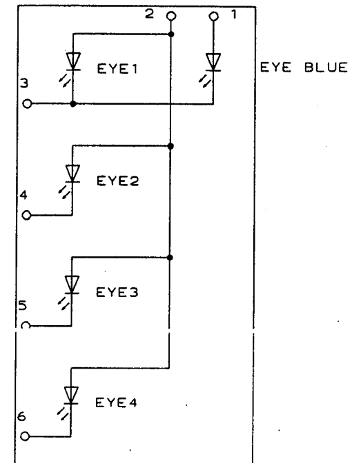
EYE LED BOARD
