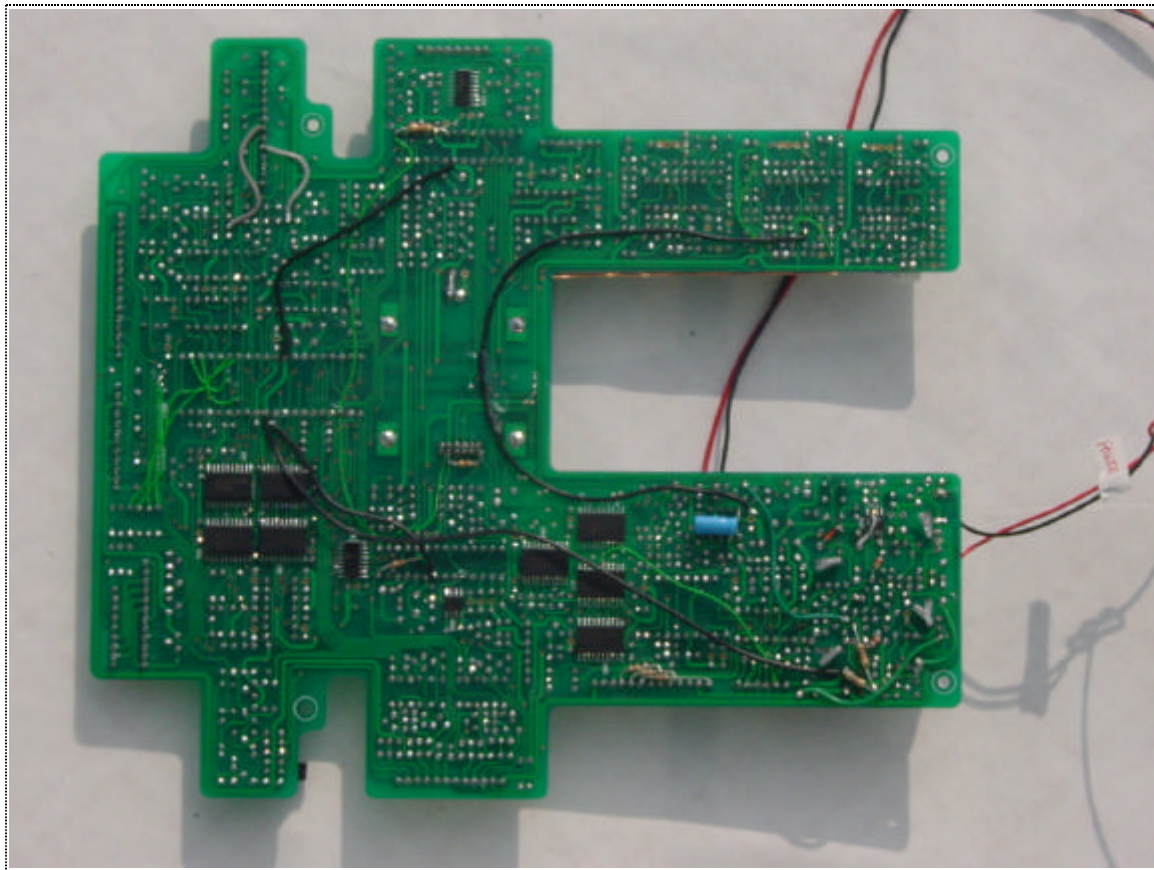
Main Control Board (Solder Side)
