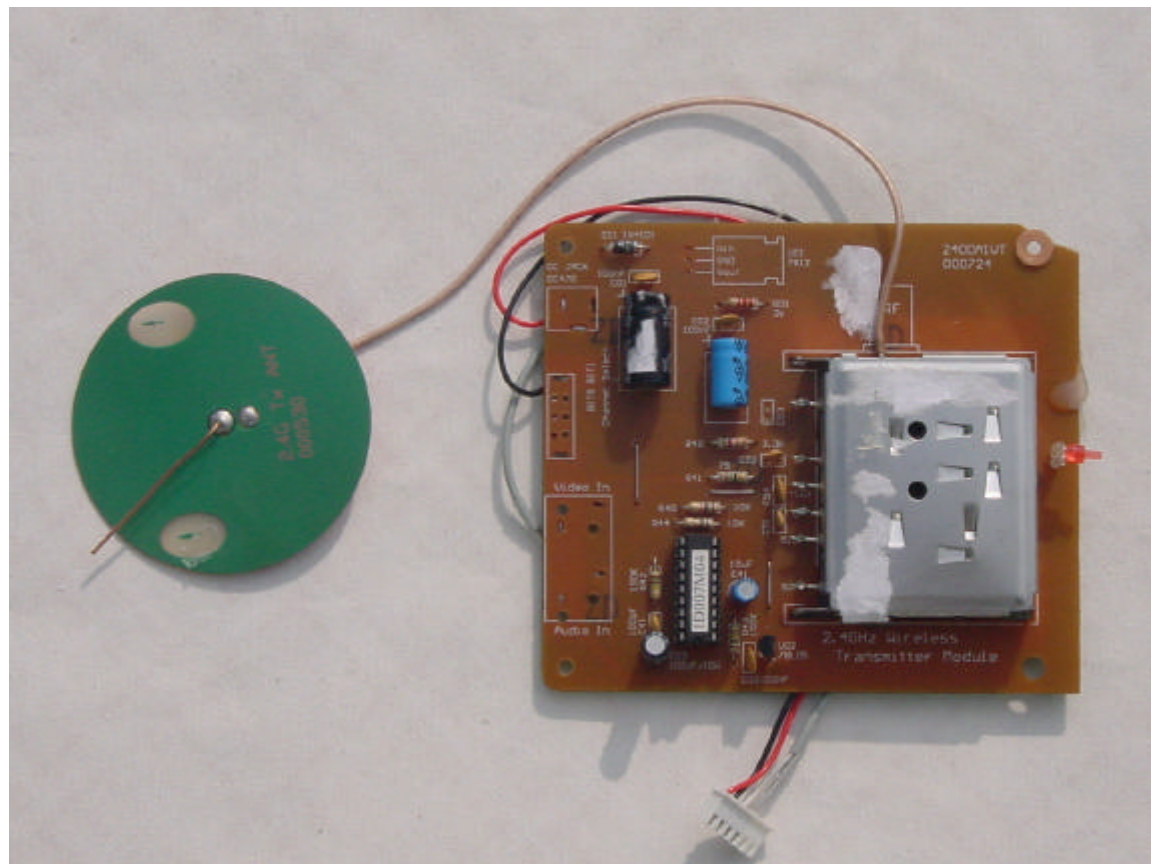
RF Module (ROBOT, Component Side)
