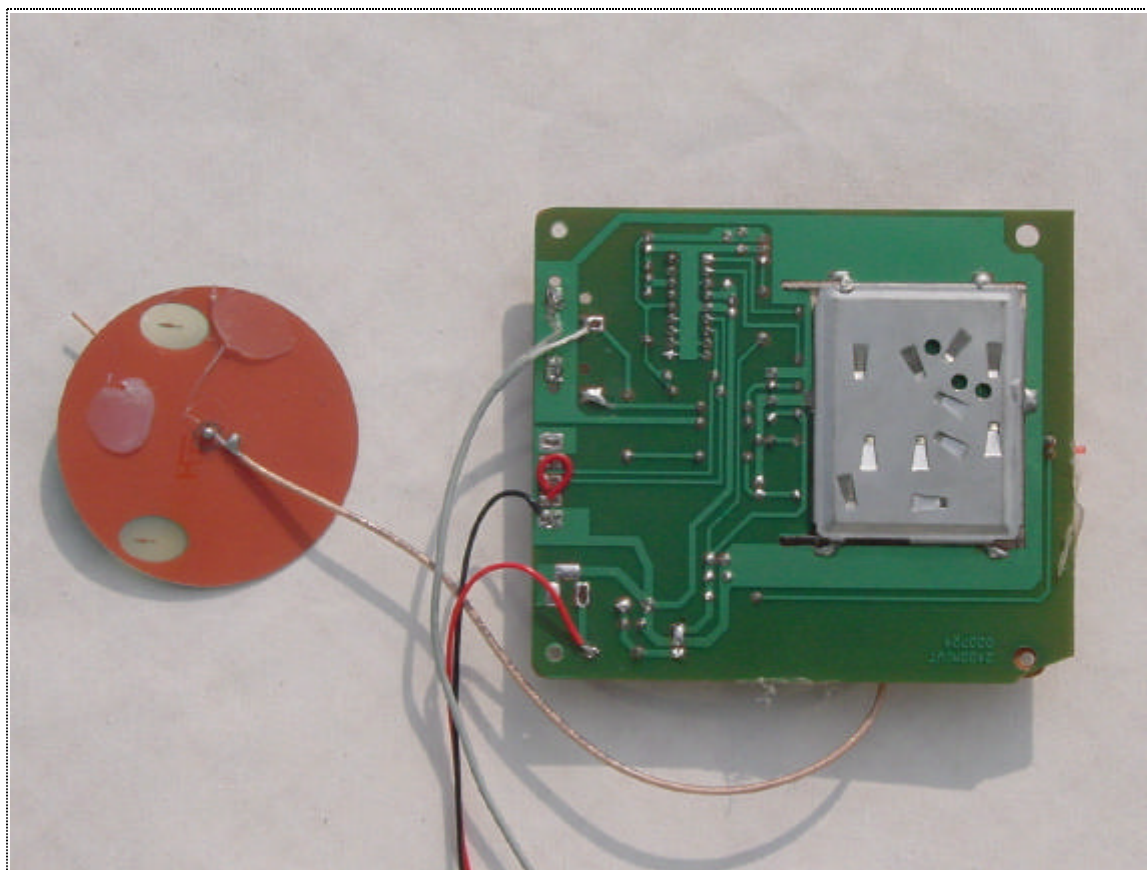
RF Module (ROBOT, Solder Side)
