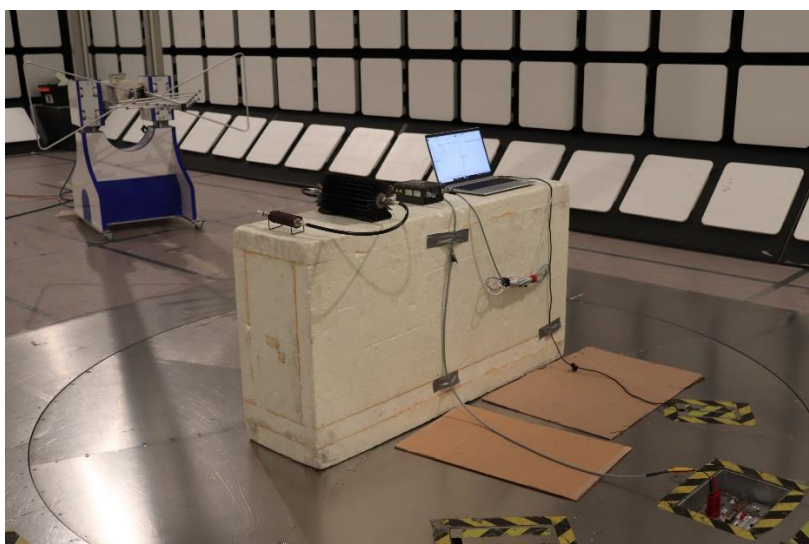
Photograph 5. Radiated Emissions 30 – 1000 MHz
