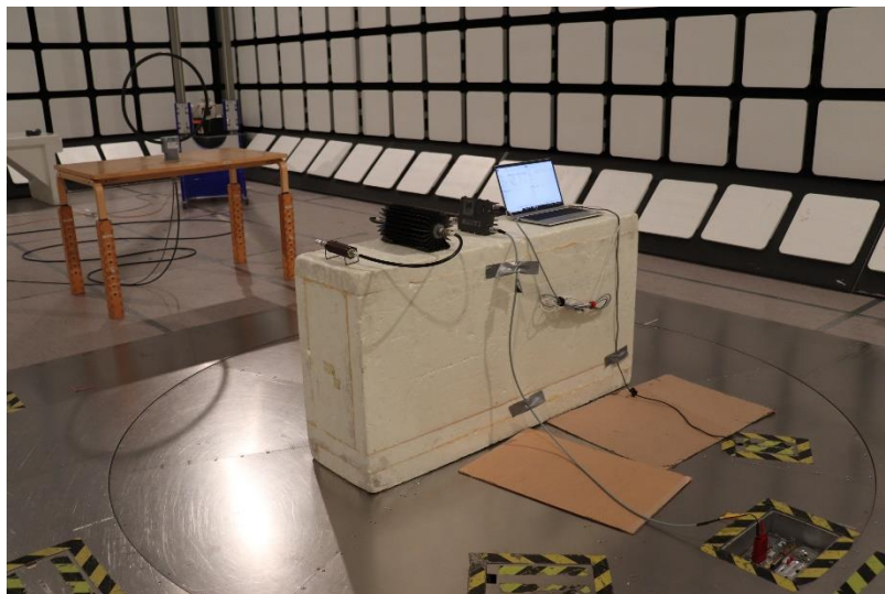
Photograph 4. Radiated Emissions 9 kHz – 30 MHz
