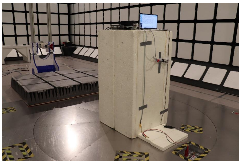
Photograph 6. Radiated Emissions 1 – 5 GHz
