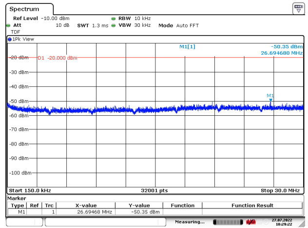
Figure 129: 150 kHz – 30 MHz
