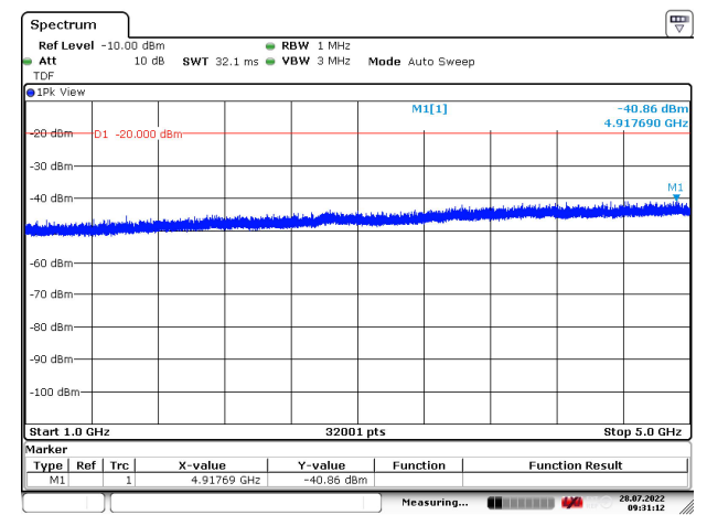
Figure 169: 1000 – 5000 MHz
