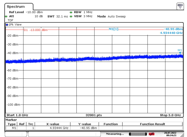
Figure 187: 1000 – 5000 MHz
