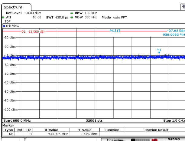
Figure 192: 600 – 1000 MHz
