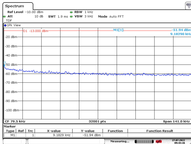
Figure 188: 9 – 150 kHz
