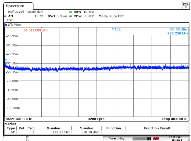
Figure 189: 150 kHz – 30 MHz
