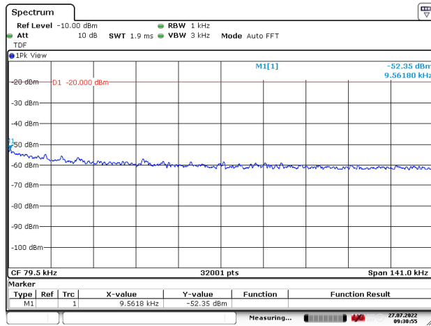
Figure 128: 9 – 150 kHz
