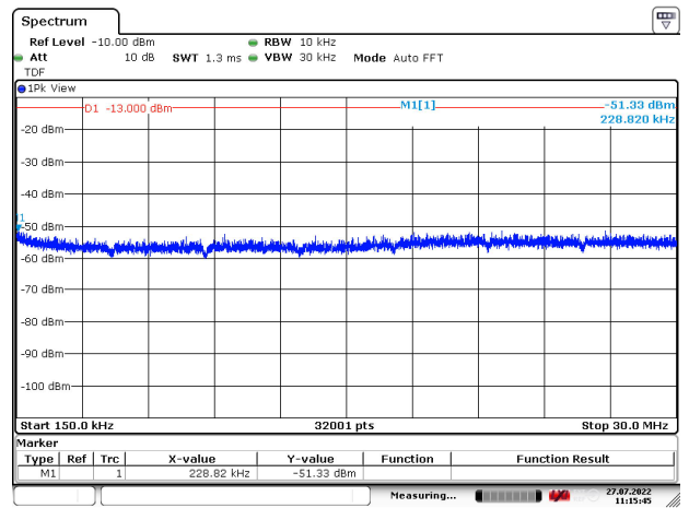
Figure 183: 150 kHz – 30 MHz
