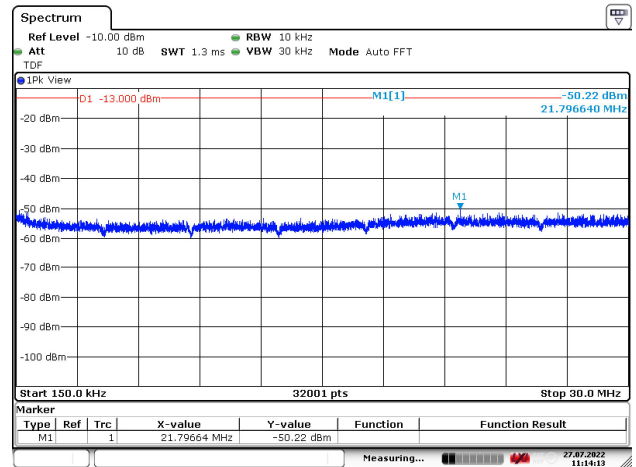
Figure 171: 150 kHz – 30 MHz
