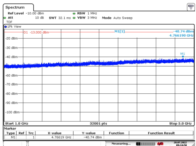
Figure 193: 1000 – 5000 MHz
