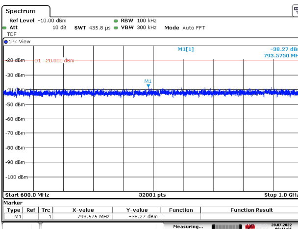
Figure 168: 600 – 1000 MHz
