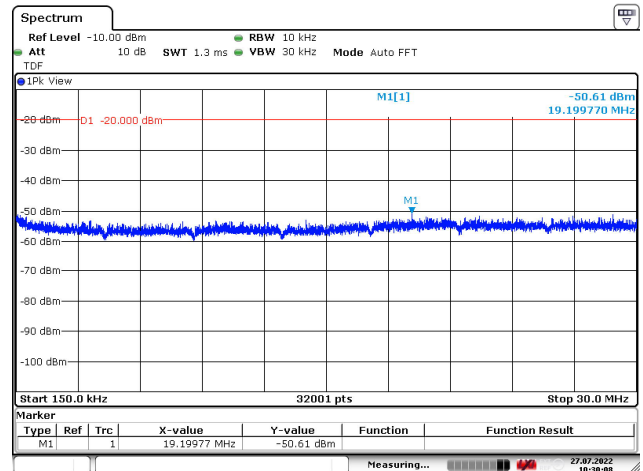
Figure 135: 150 kHz – 30 MHz
