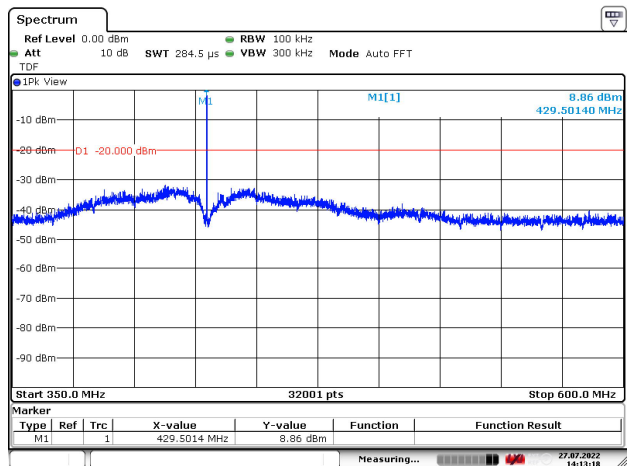
Figure 131: 350 – 600 MHz
