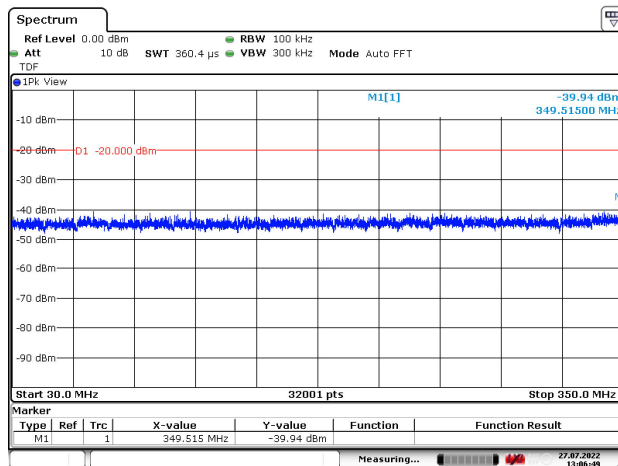
Figure 130: 30 – 350 MHz
