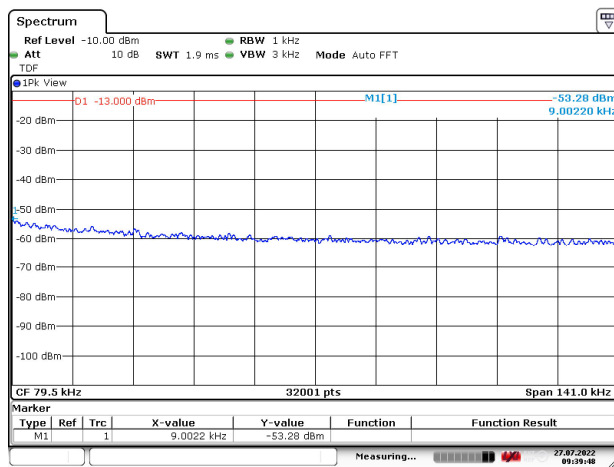
Figure 170: 9 – 150 kHz
