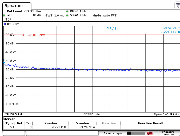
Figure 134: 9 – 150 kHz
