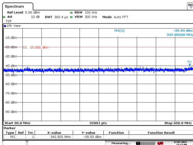
Figure 160: 30 – 350 MHz
