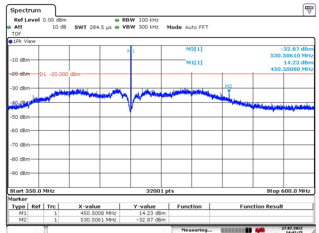
Figure 161: 350 – 600 MHz
