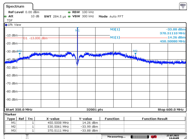
Figure 185: 350 – 600 MHz
