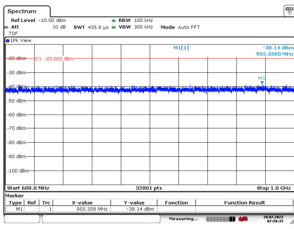
Figure 96: 600 – 1000 MHz
