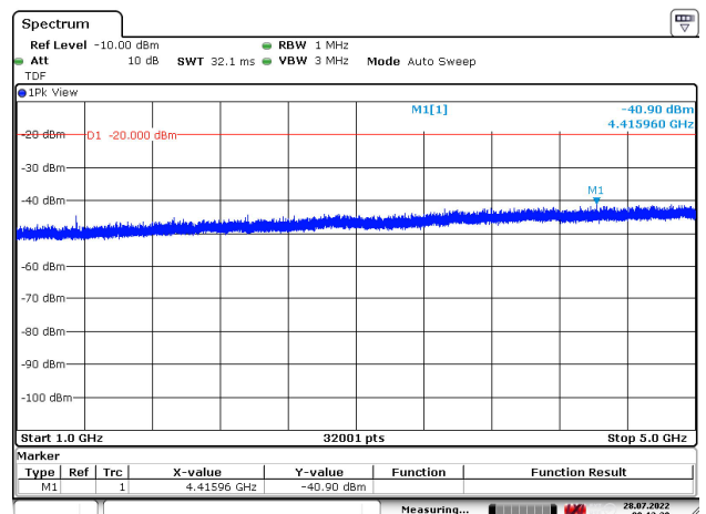
Figure 67: 1000 – 5000 MHz
