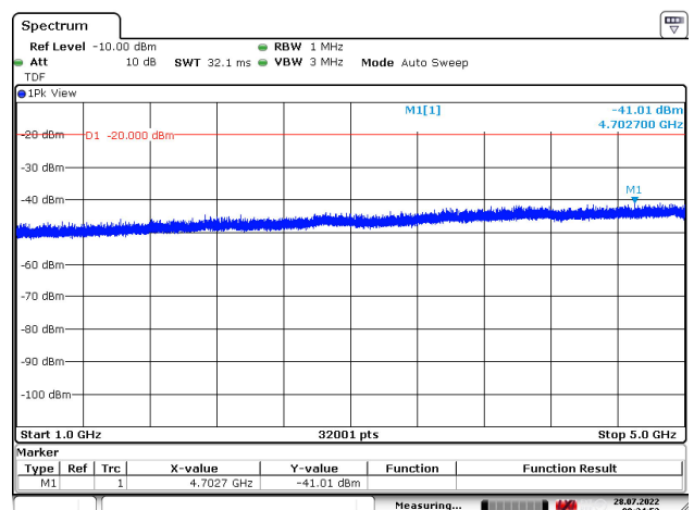
Figure 127: 1000 – 5000 MHz
