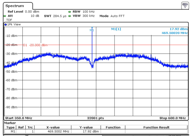
Figure 95: 350 – 600 MHz
