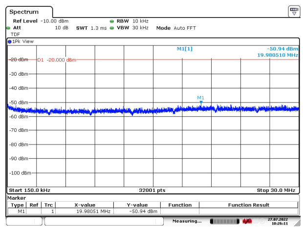
Figure 111: 150 kHz – 30 MHz
