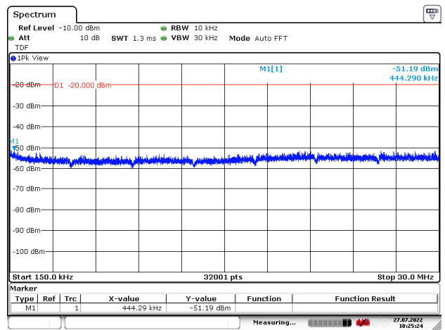
Figure 105: 150 kHz – 30 MHz
