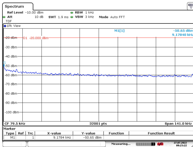
Figure 92: 9 – 150 kHz
