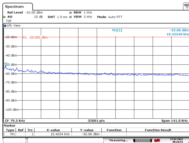
Figure 122: 9 – 150 kHz
