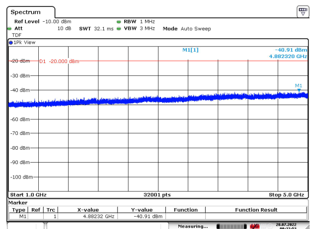
Figure 115: 1000 – 5000 MHz
