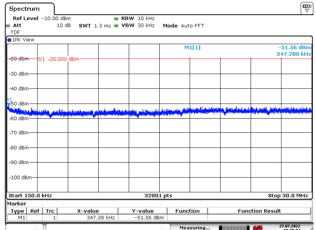
Figure 123: 150 kHz – 30 MHz
