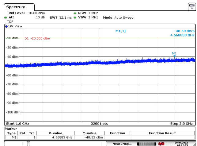
Figure 109: 1000 – 5000 MHz
