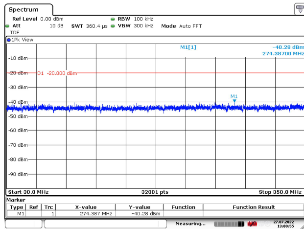
Figure 94: 30 – 350 MHz
