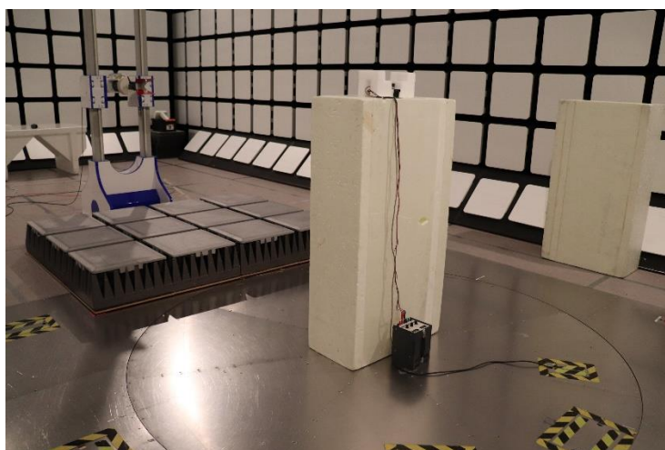
Photograph 5. Radiated Emissions above 1 GHz
