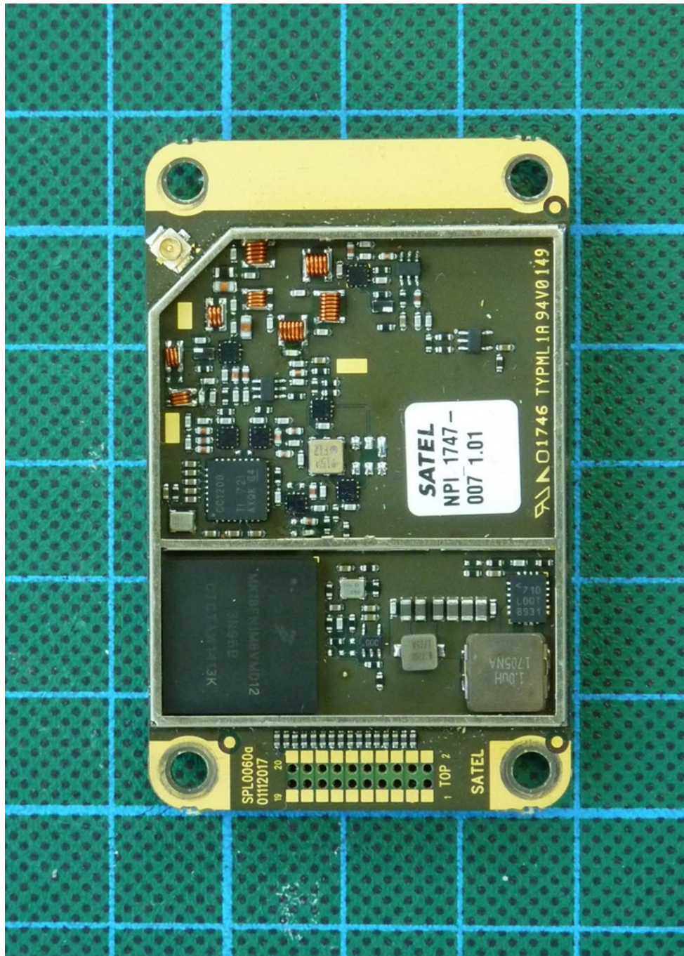
172629_10.jpg: EUT – top view, shielding removed
