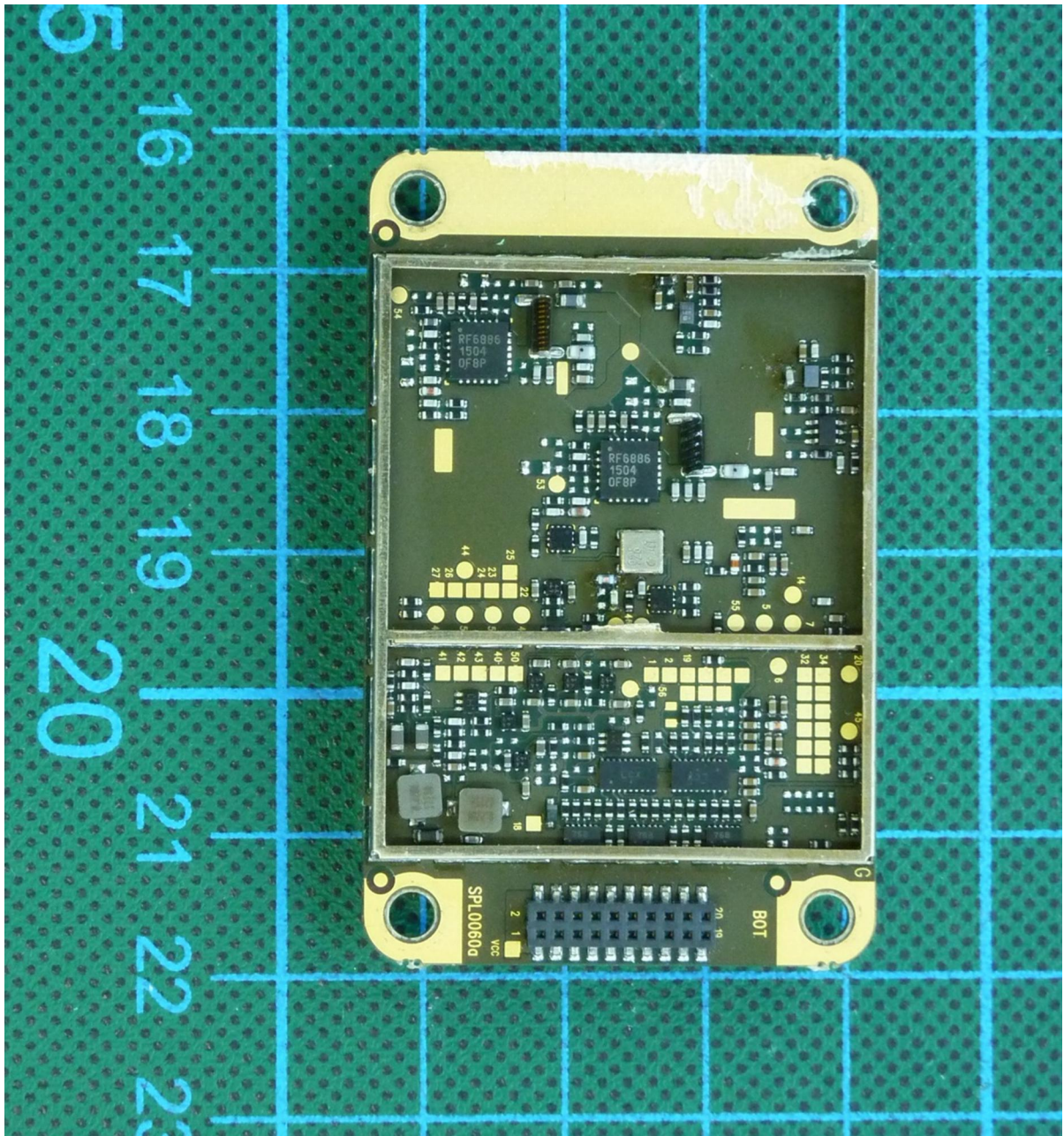
172629_11.jpg: EUT – bottom view, shielding removed
