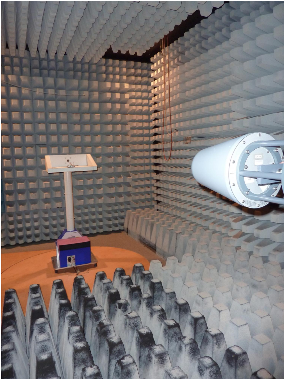
172629_02.JPG: Test setup - Radiated emission (fully anechoic chamber)
