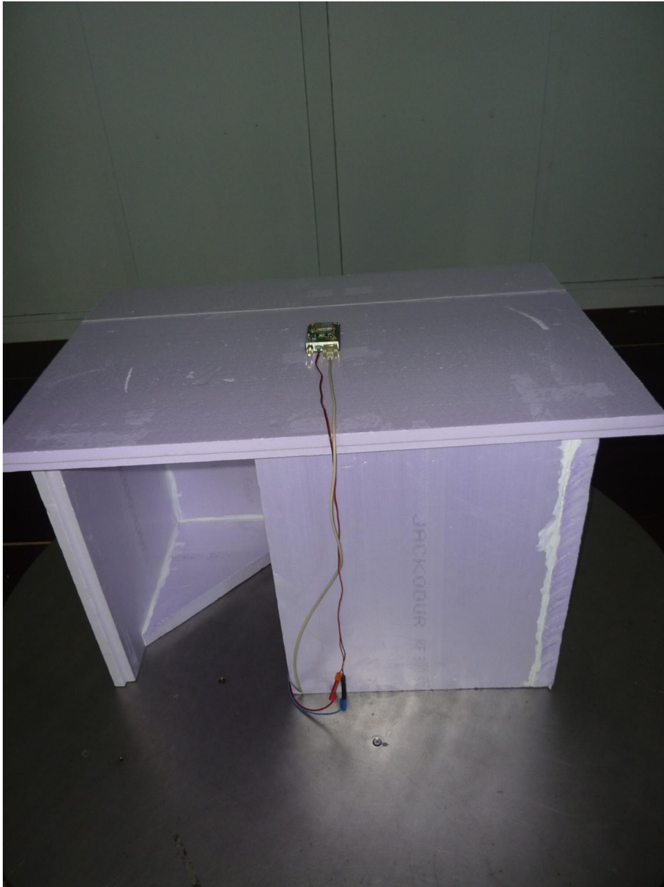
172629_03.JPG: Test setup - Radiated emission (OATS)
