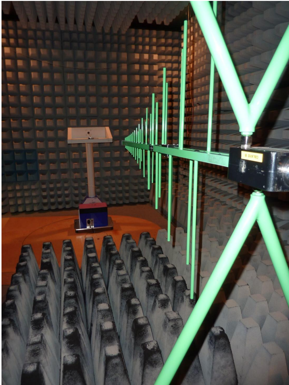
172629_01.JPG: Test setup - Radiated emission (fully anechoic chamber)
