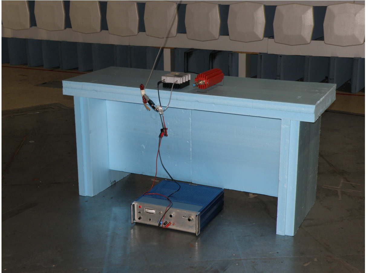
Photograph 1. Radiated spurious emission test.
