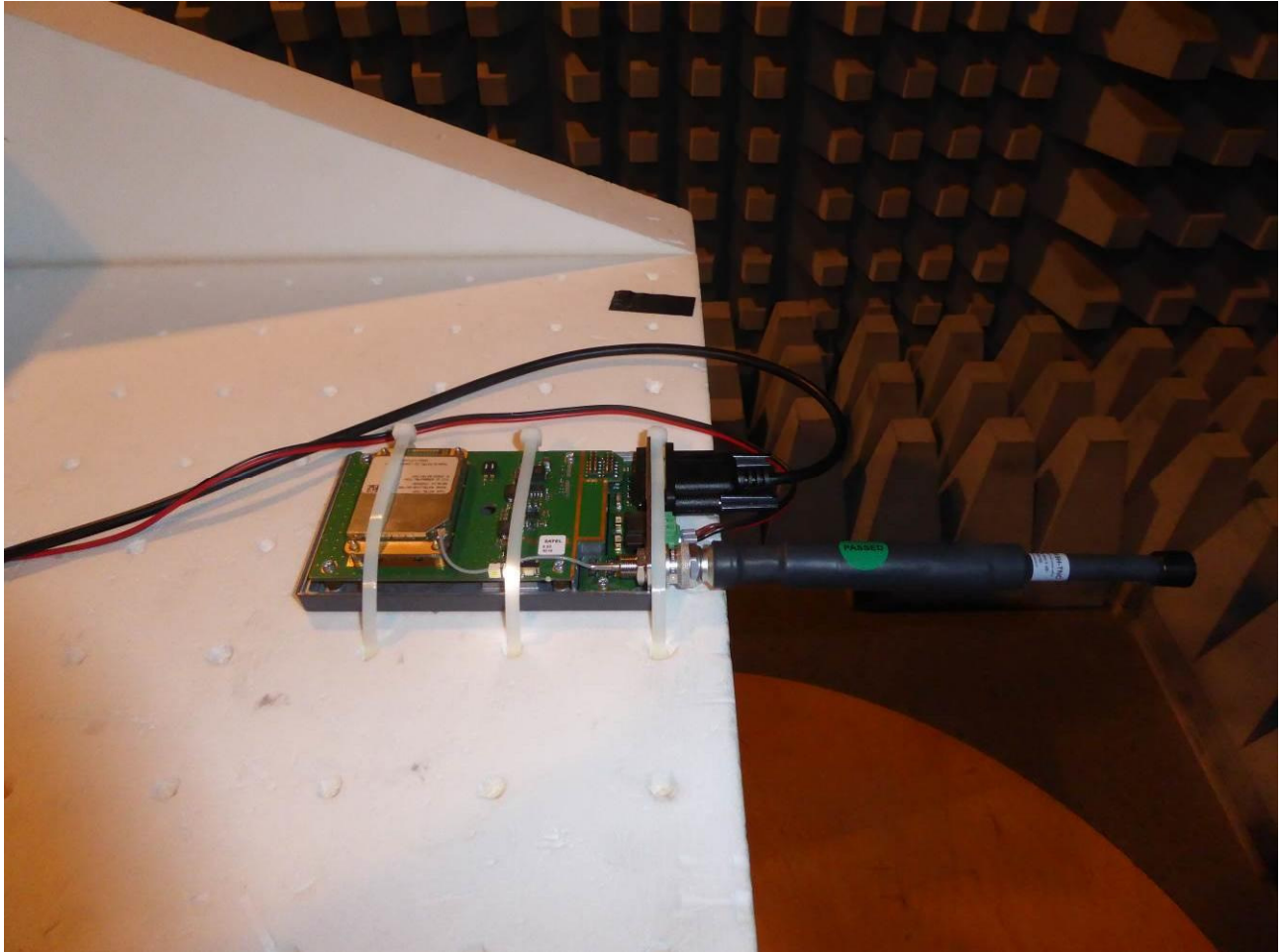
170226_03: Test setup CAH antenna - Radiated emission anechoic chamber
