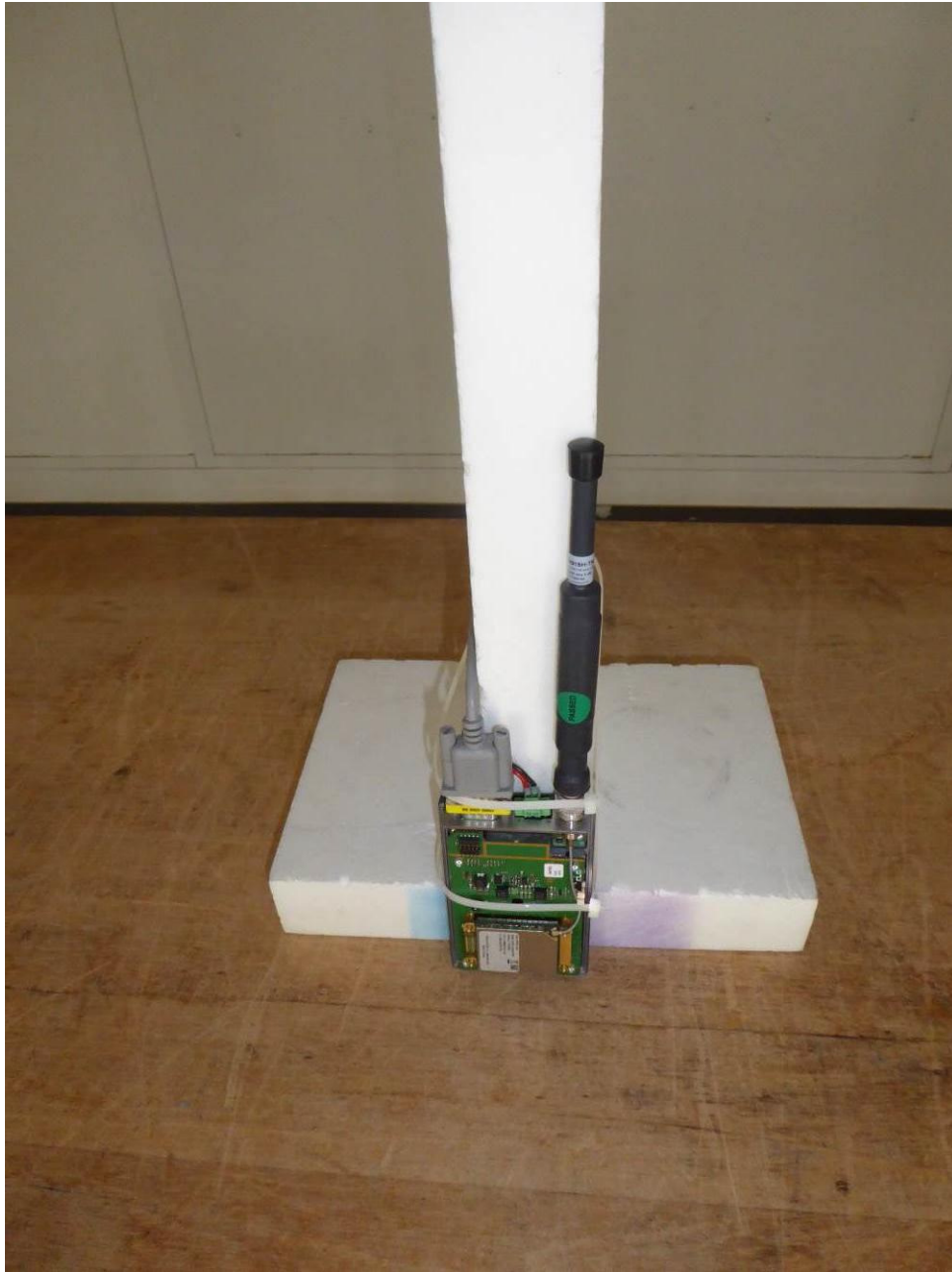
170226_09: Test setup CAH antenna - Radiated emission open area test site
