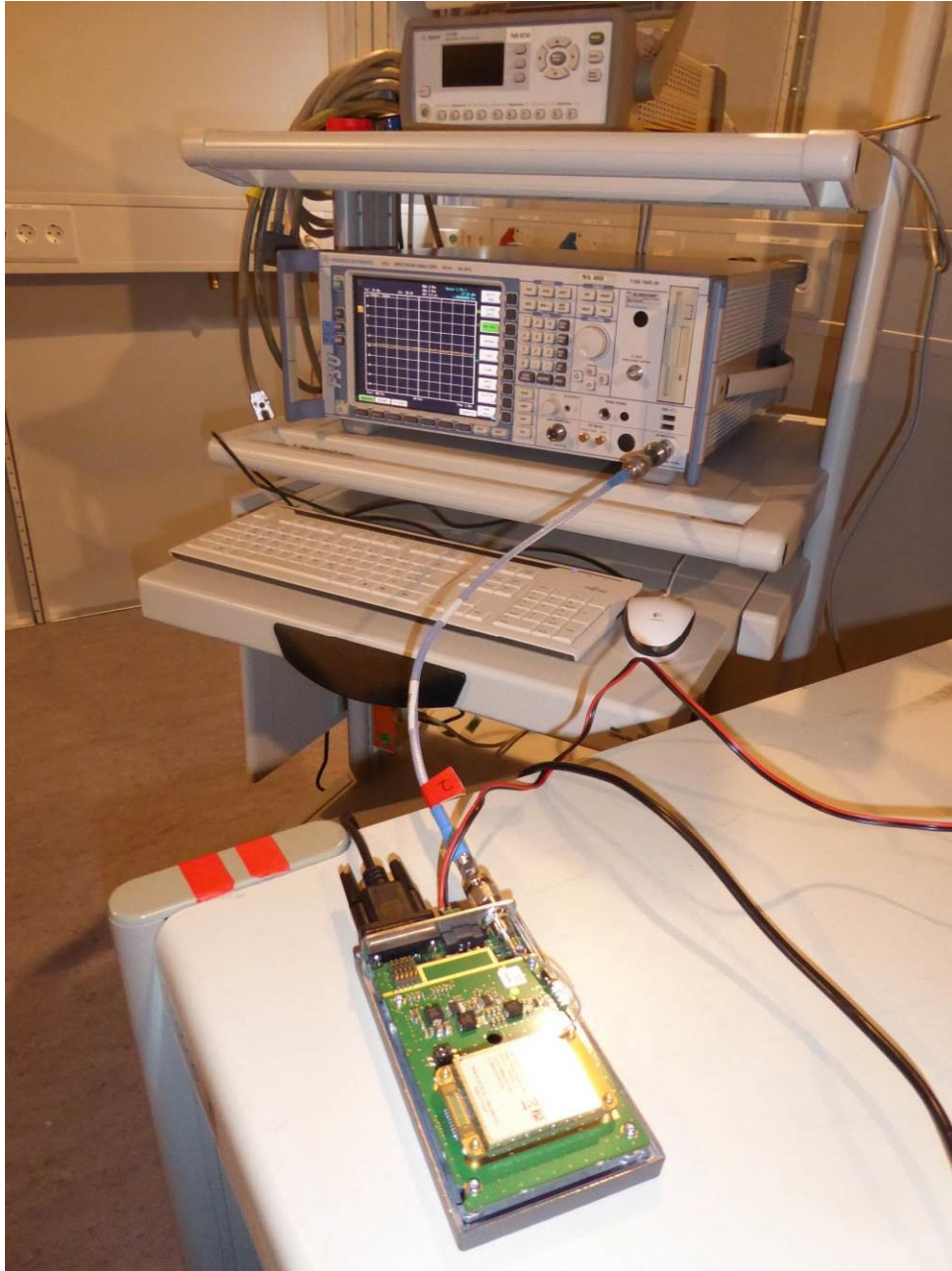
170226_01.JPG: Test setup - conducted tests
