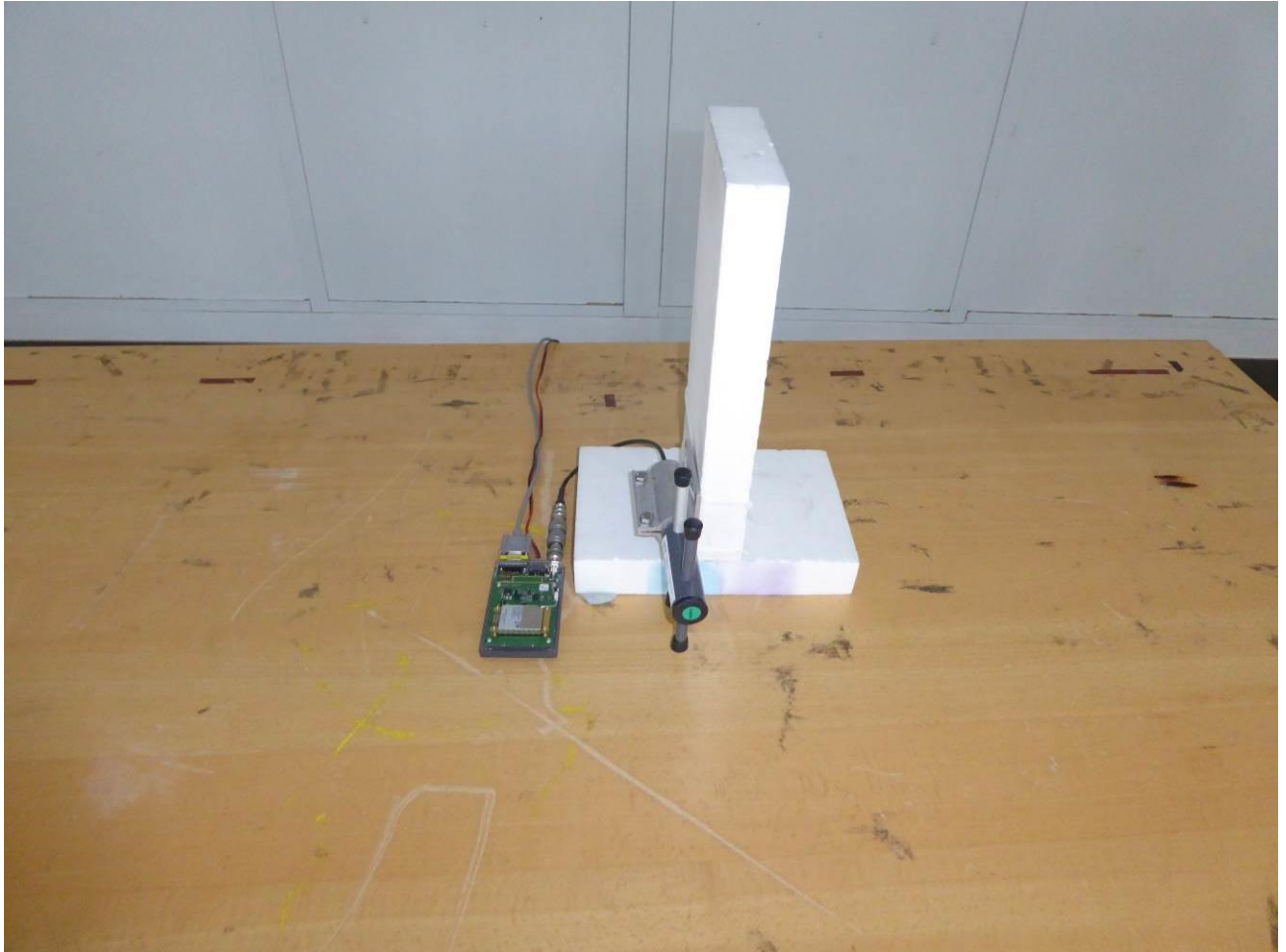
170226_08: Test setup CAY antenna - Radiated emission open area test site
