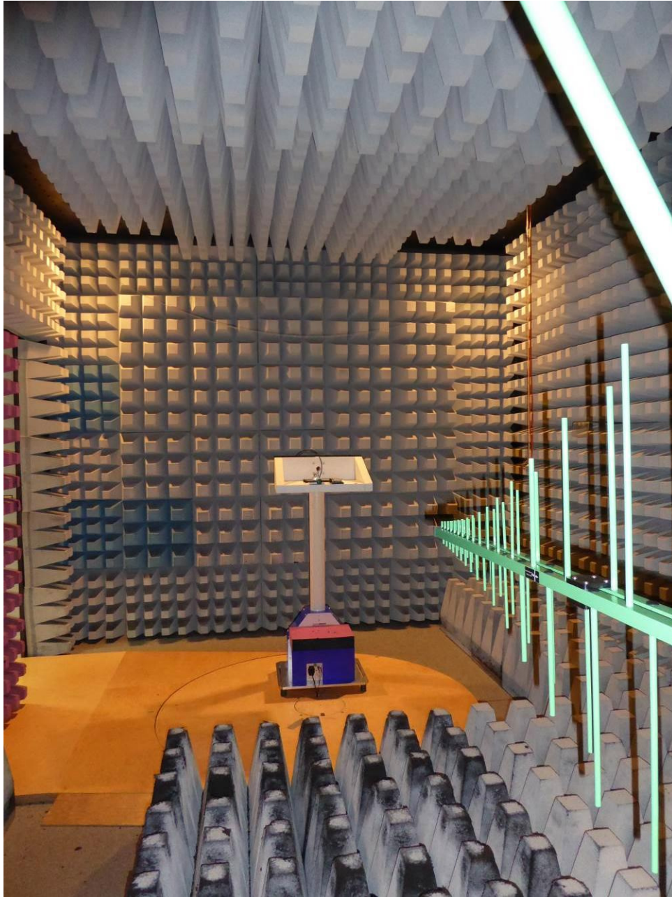
170226_07: Test setup CAY antenna - Radiated emission anechoic chamber
