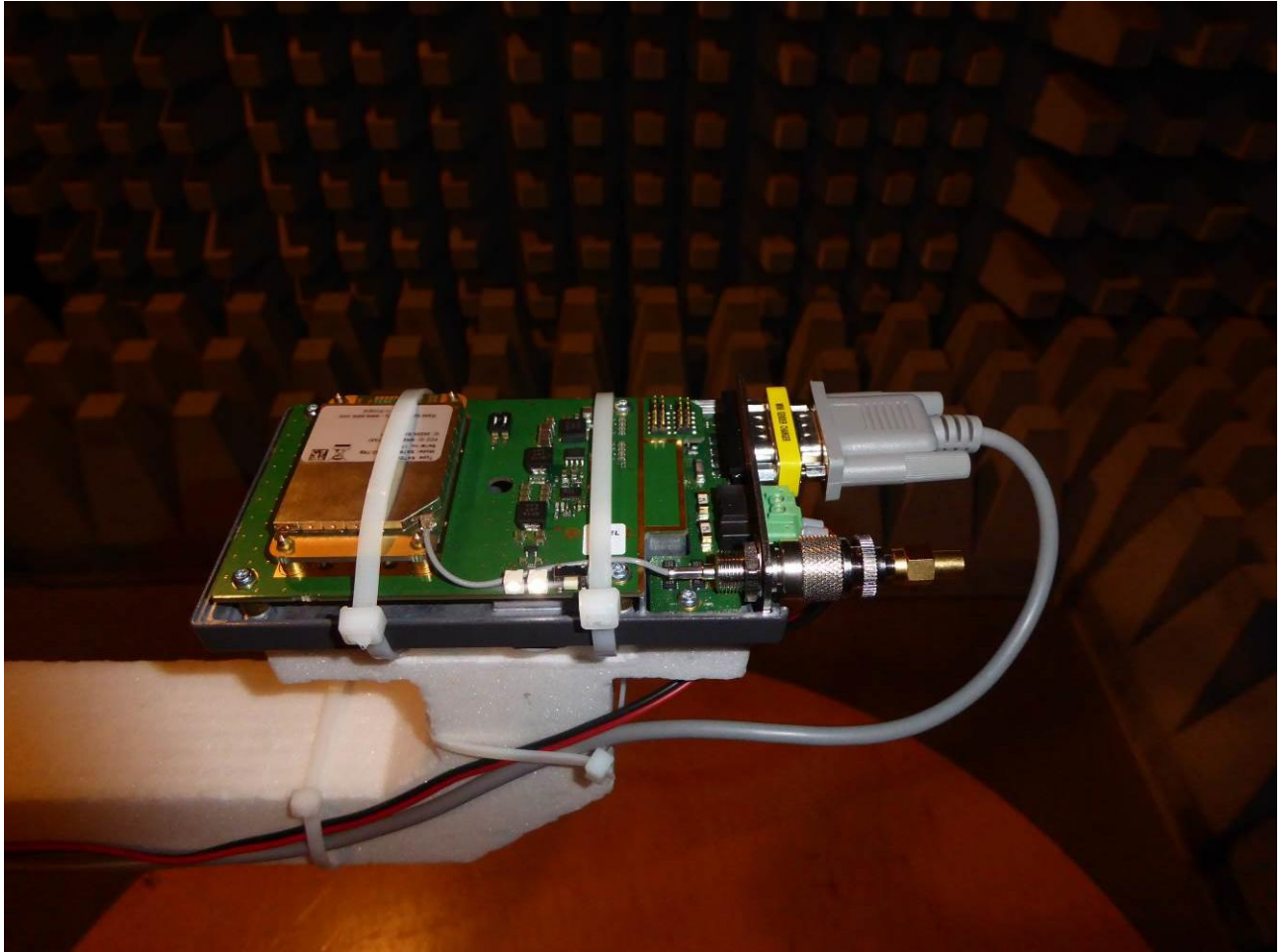
170226_04: Test setup antenna port terminated - Radiated emission anechoic chamber
