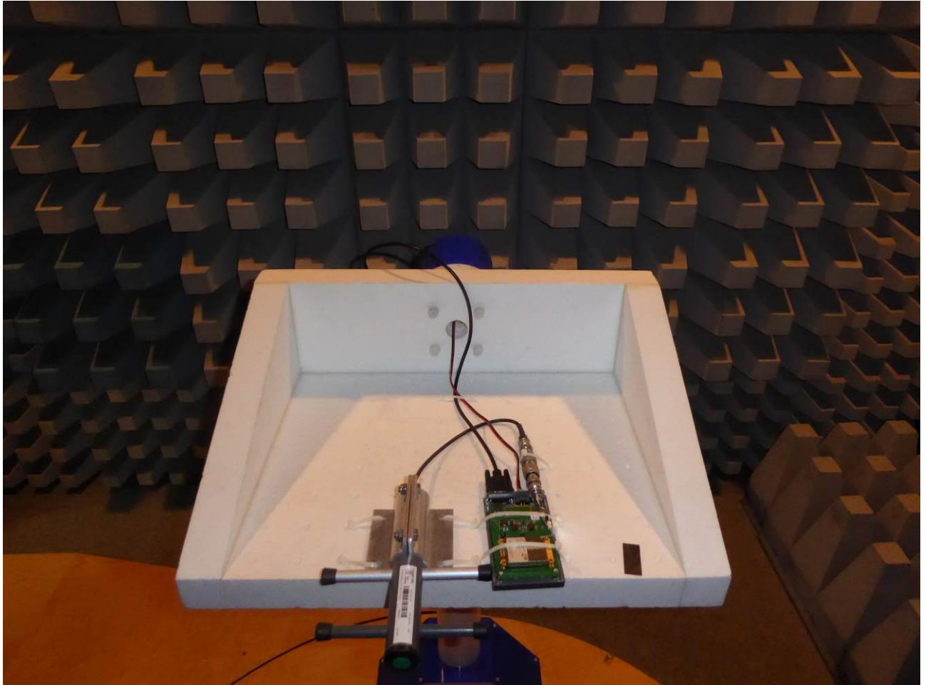
170226_02: Test setup CAY antenna - Radiated emission anechoic chamber
