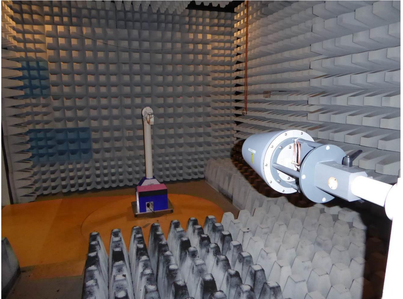
170226_10: Test setup antenna port terminated - Radiated emission anechoic chamber
