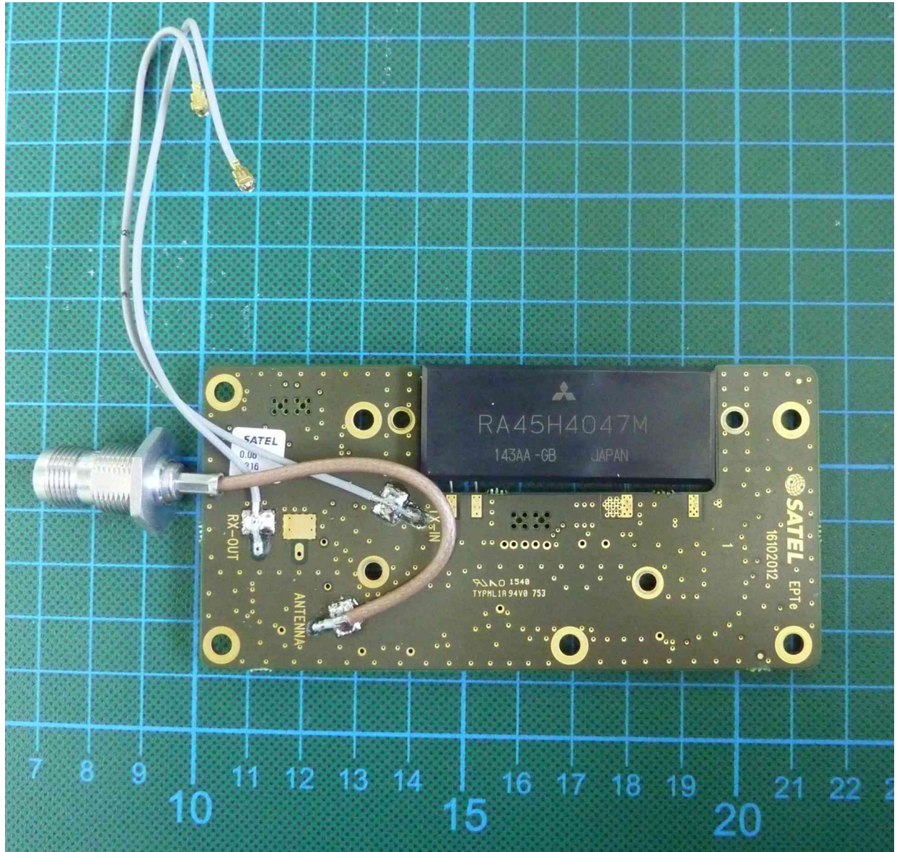
160575_22.jpg: PA board, top view
