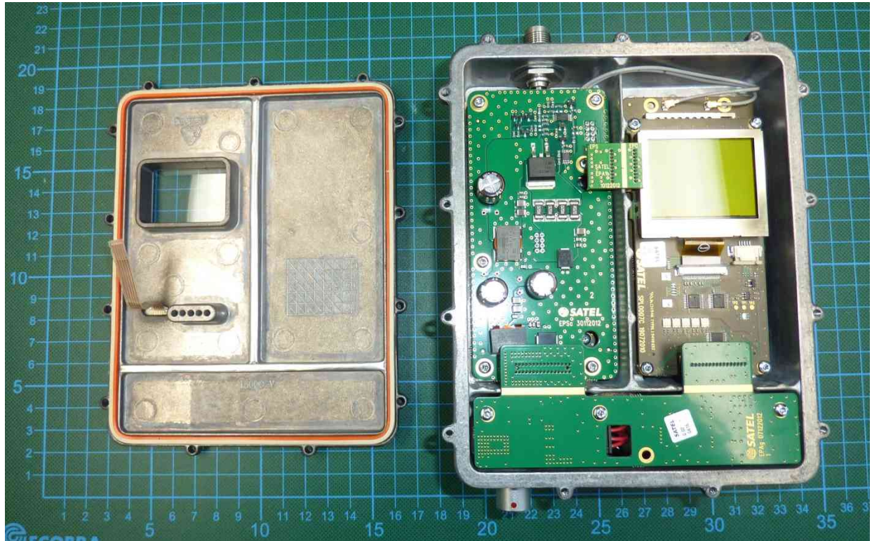
160575_11.jpg: EUT, cabinet opened
