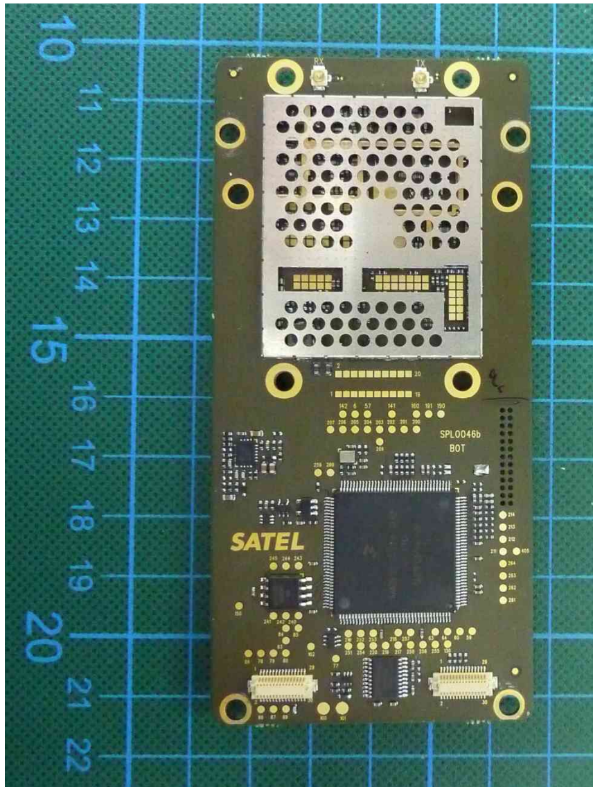
160575_25.jpg: Modem board, bottom view
