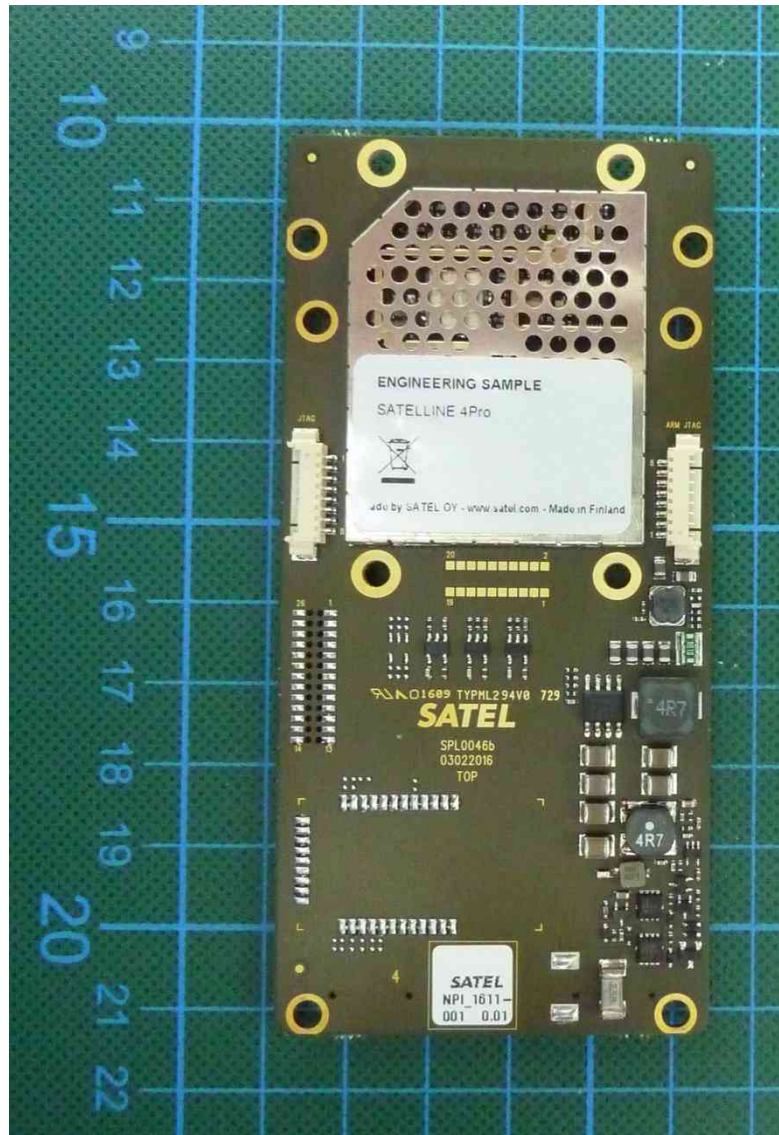
160575_24.jpg: Modem board, top view
