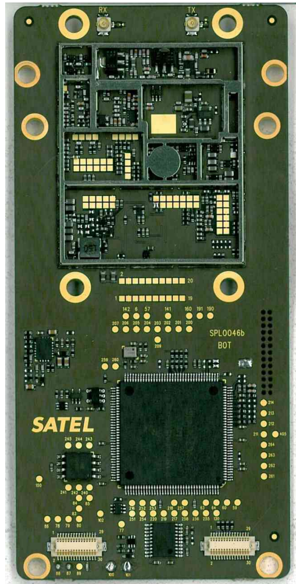
160575_26.jpg: Modem board, top view, shielding removed (Photo supplied by the applicant)
