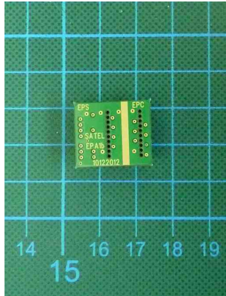
160575_17.jpg: Connector board, top view
