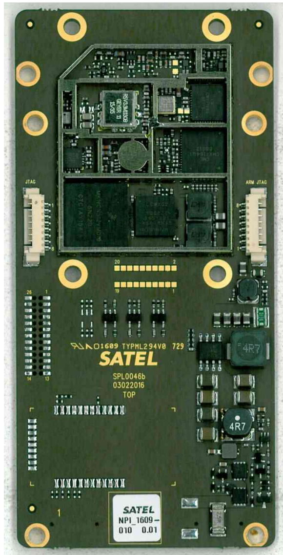
160575_27.jpg: Modem board, bottom view, shielding removed (Photo supplied by the applicant)
