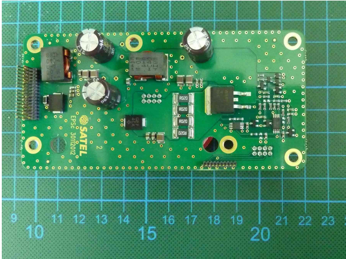
160575_15.jpg: DC power supply board, top view
