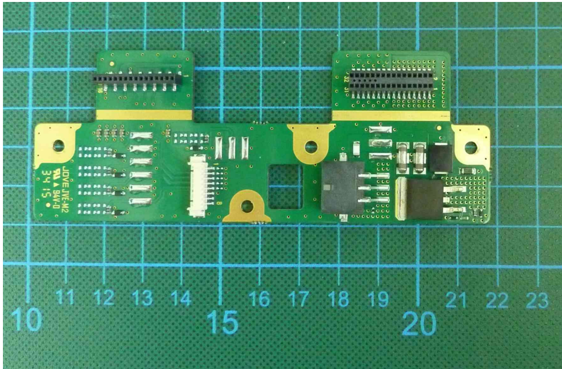
160575_13.jpg: DC / RS232 connection board, top view
