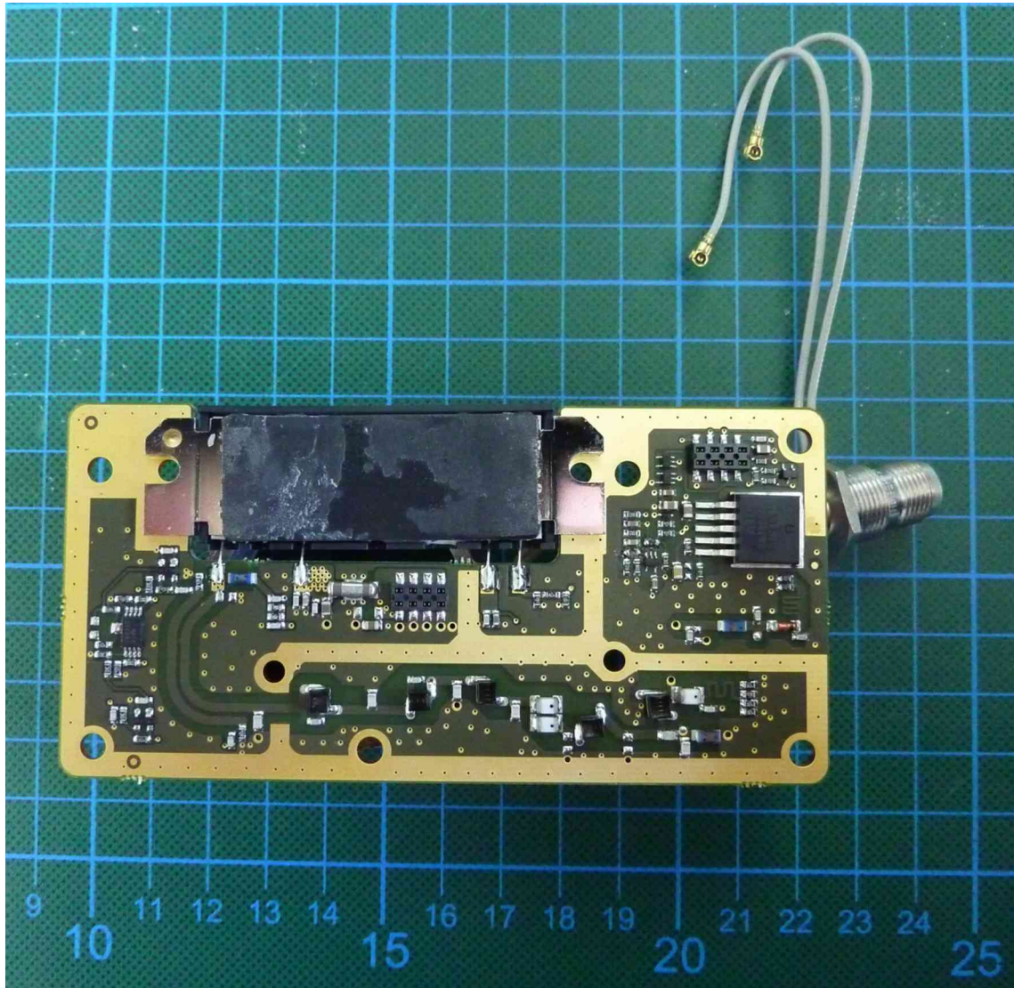
160575_23.jpg: PA board, bottom view
