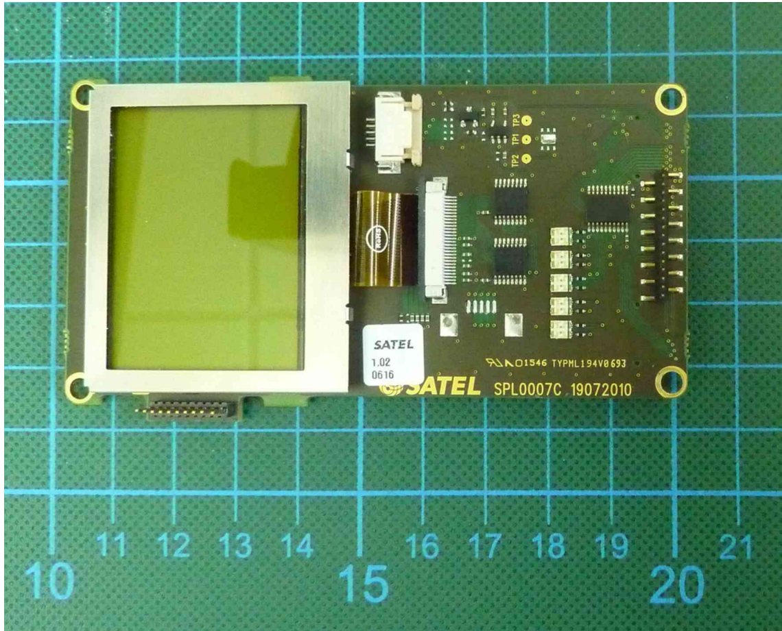
160575_19.jpg: Display board, top view
