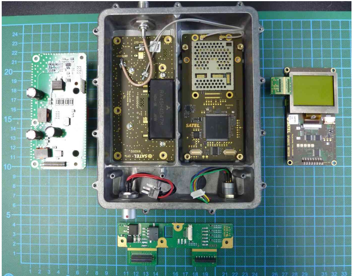
160575_12.jpg: EUT – DC power supply board , display board and DC / RS 232 board removed
