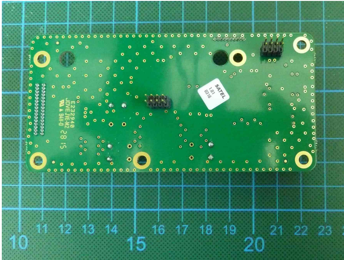
160575_16.jpg: DC power supply board, bottom view
