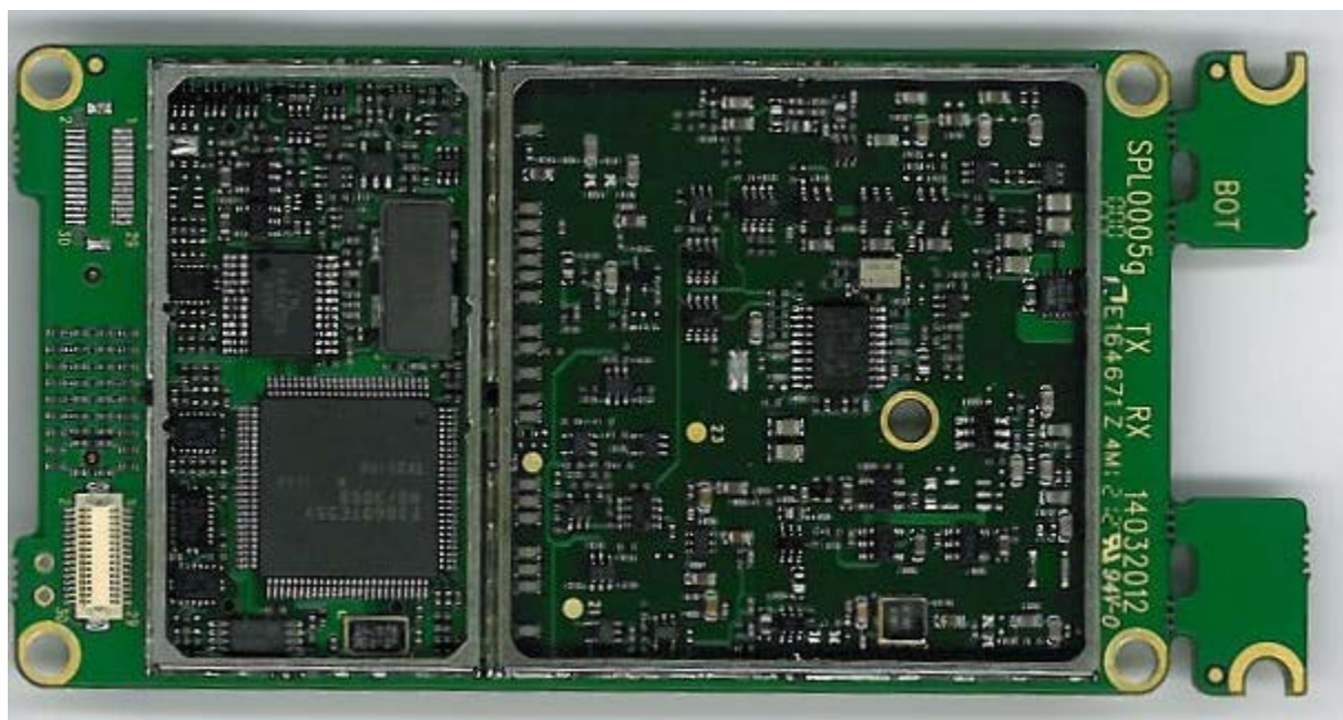
Photo1: SATELLINE-M3-TR1 internal view from bottom
