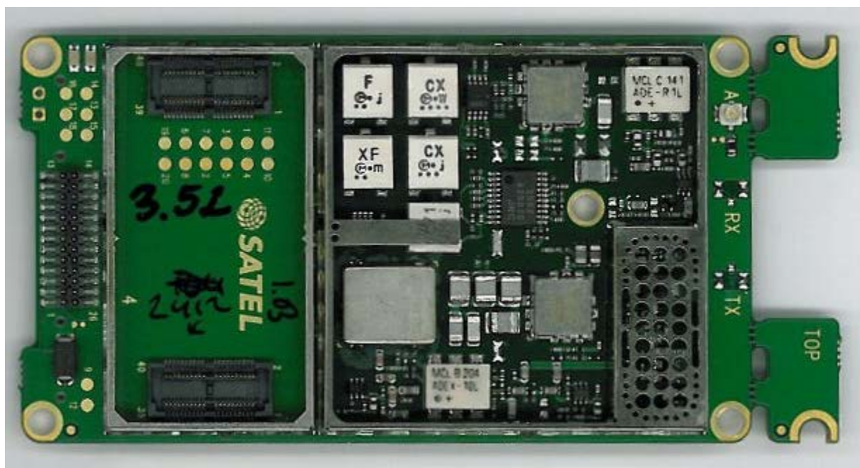
Photo2: SATELLINE-M3-TR1 internal view from top
