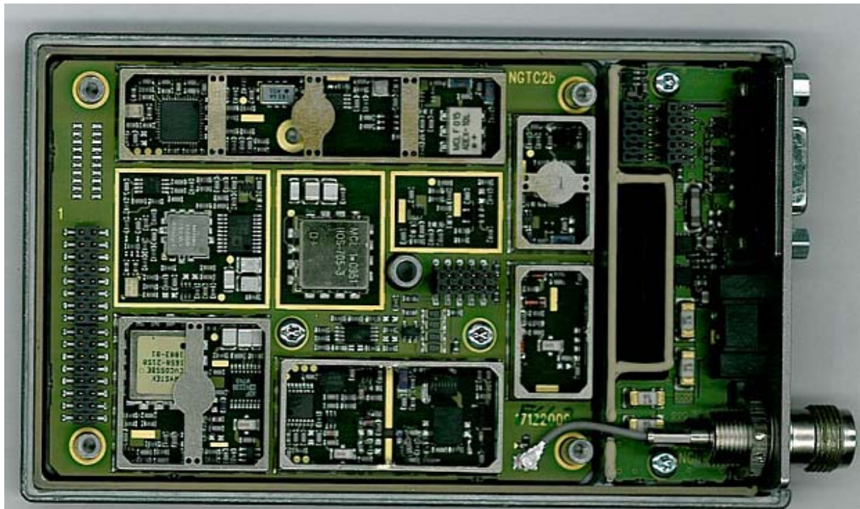
Radio Board NGTC2b_TV04 = 470 - 520 MHz
