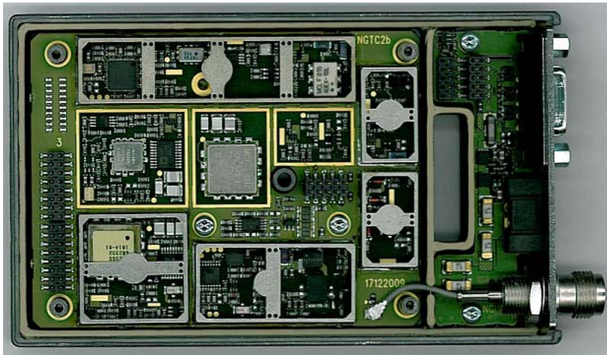
Radio board NGTC2b_TV02 = 406,1 - 445 MHz
