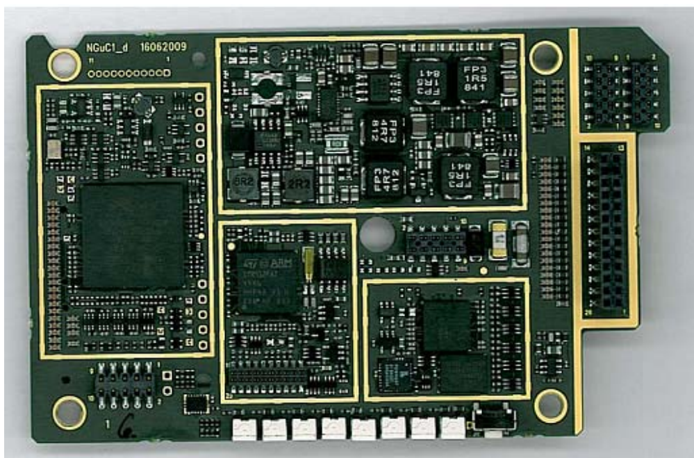
Logic board NGuC1_d (same to all versions)
