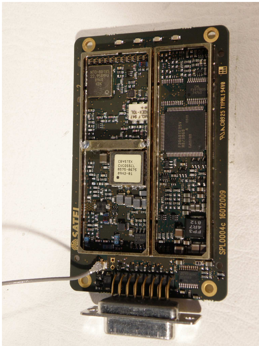
Photograph 3.: Upside without RF shield
