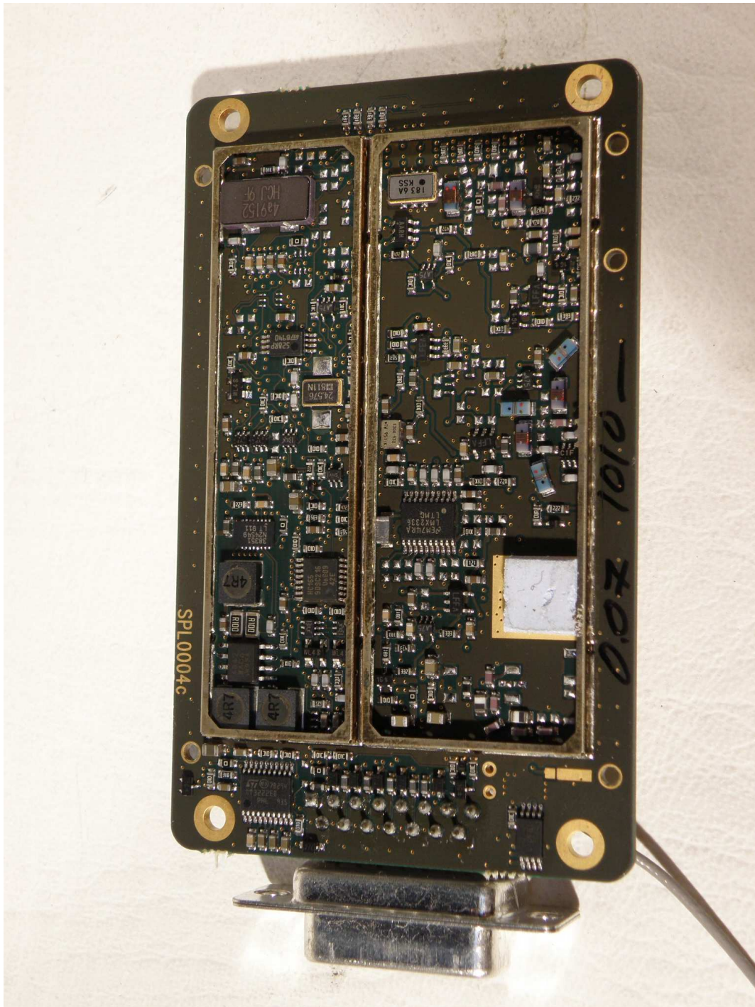
Photograph 4.: Downside without RF shield
