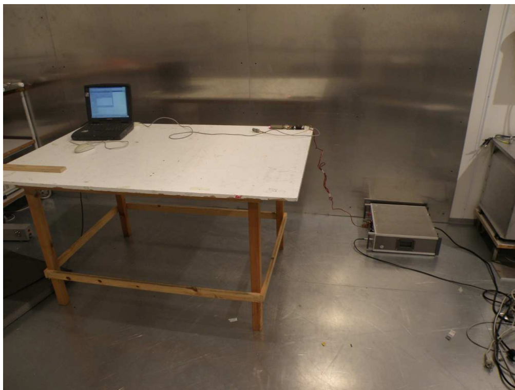
Photograph 1. Conducted disturbance at mains ports emission test.
