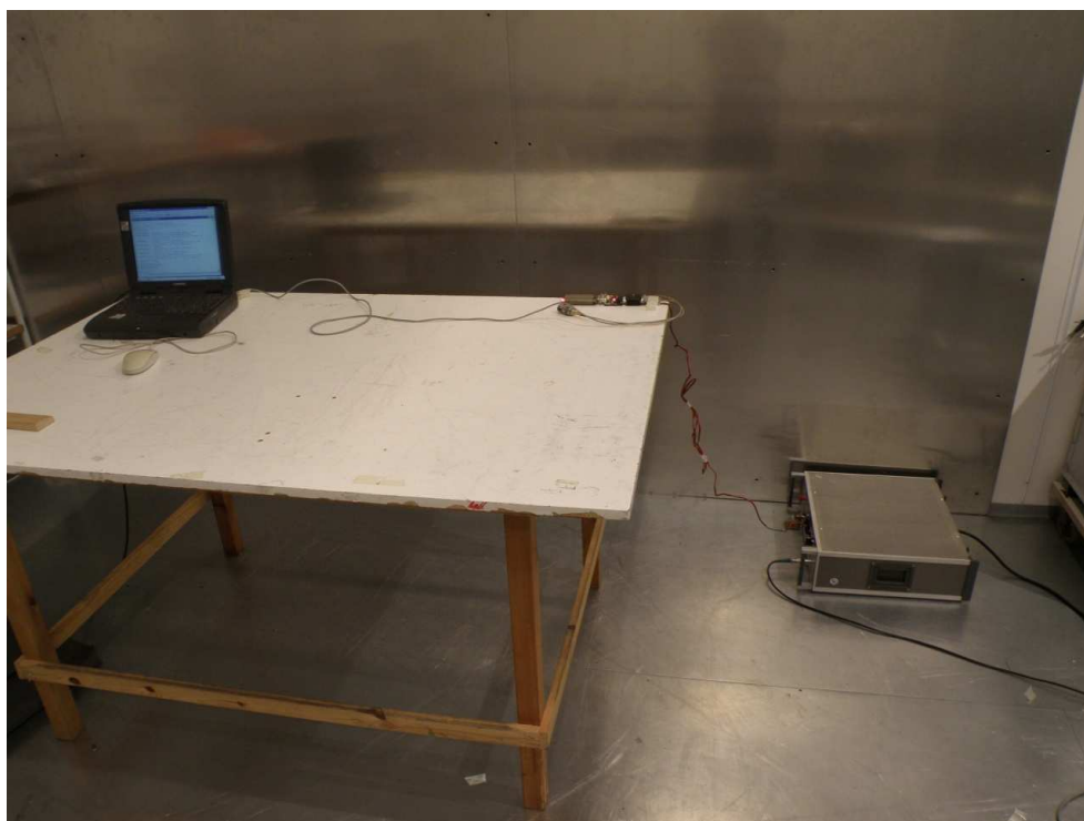
Photograph 2. Conducted disturbance at mains ports emission test.
