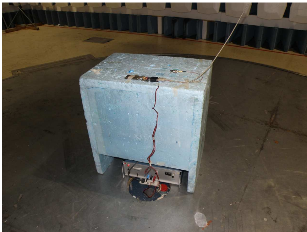
Photograph 1. Radiated disturbance emission test.
