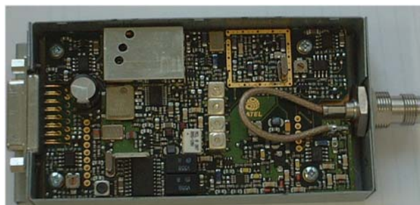
Picture 2. Inside of the SATELLINE-3ASm
