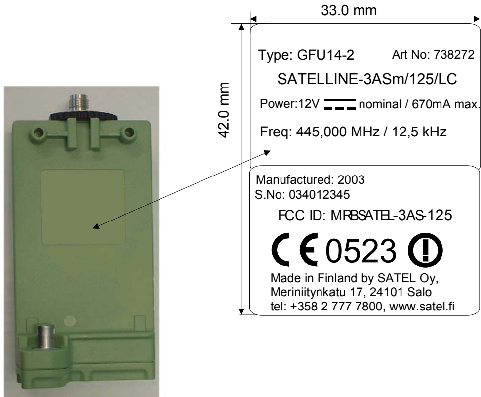
Picture 5. Bottom view of the SATELLINE-3ASm/125/LC with label
