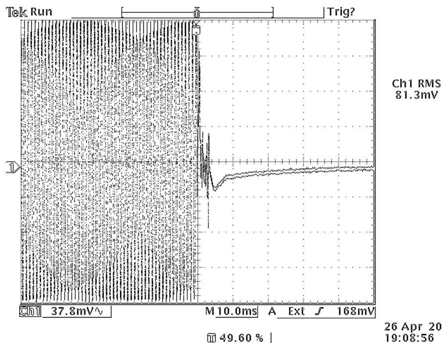
Fig. 11. Transmitter switched ON at +20 °C. (12.5 kHz ch. sp.)
