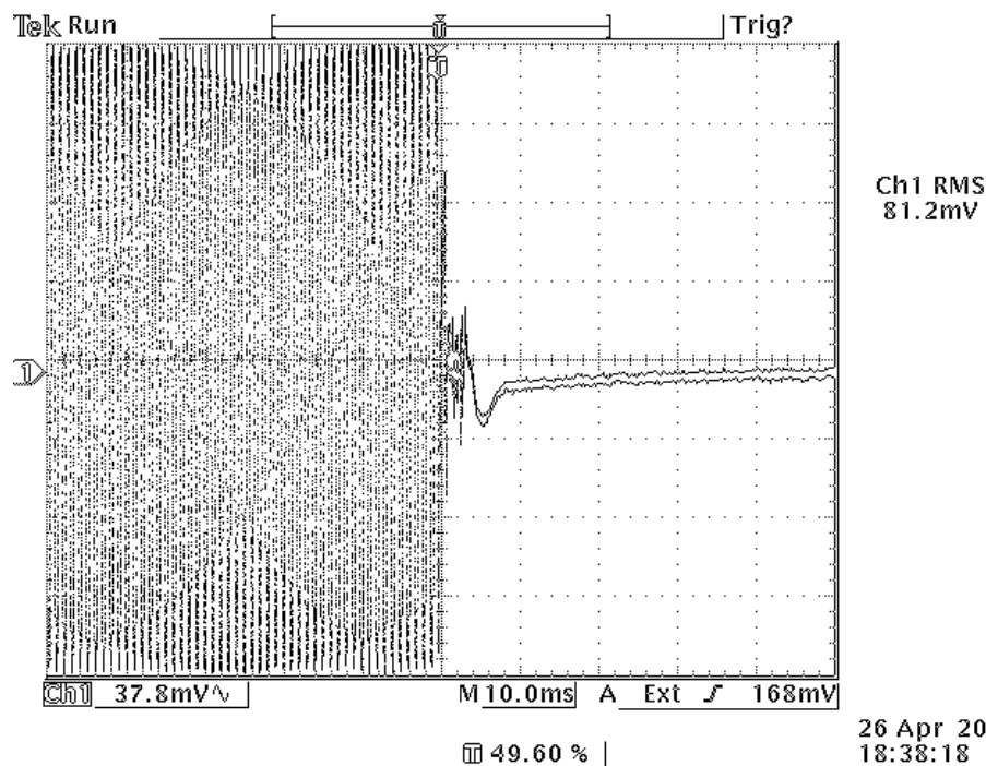
Fig. 7. Transmitter switched ON at 0 °C. (12.5 kHz ch. sp.)
