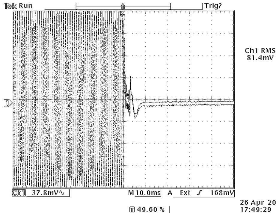
Fig. 1. Transmitter switched ON at -30 °C. (12.5 kHz ch. sp.)
