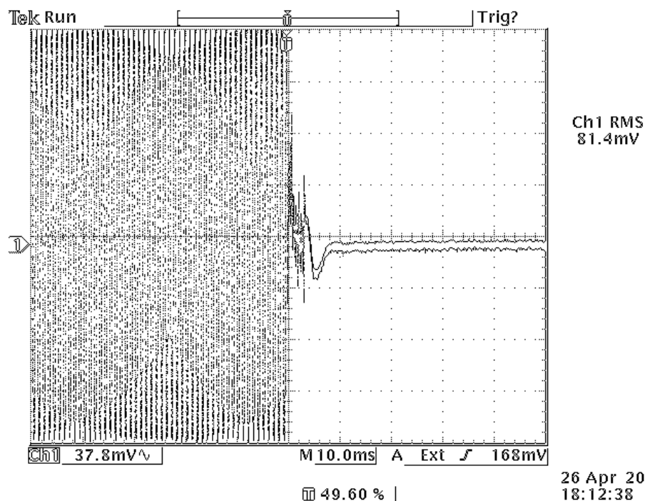
Fig. 3. Transmitter switched ON at -20^{\circ}\text{C} . (12.5 kHz ch. sp.)
