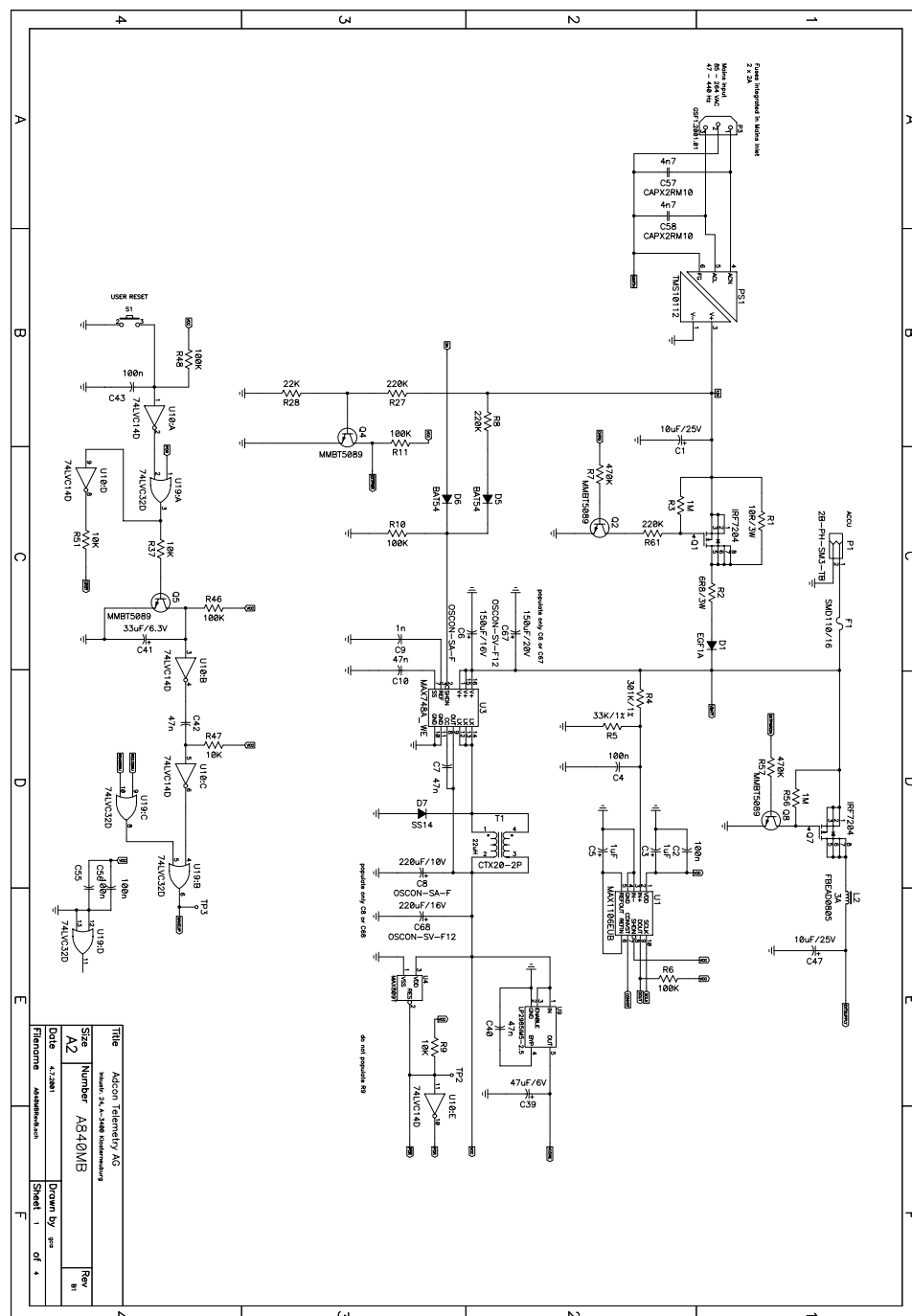
Figure 4. A840 Power Supply
