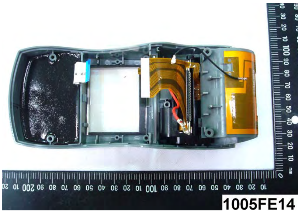
(32) EUT Photo
