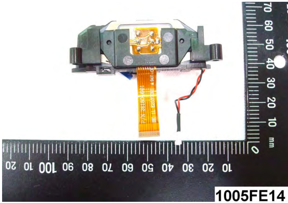
(23) EUT Photo
