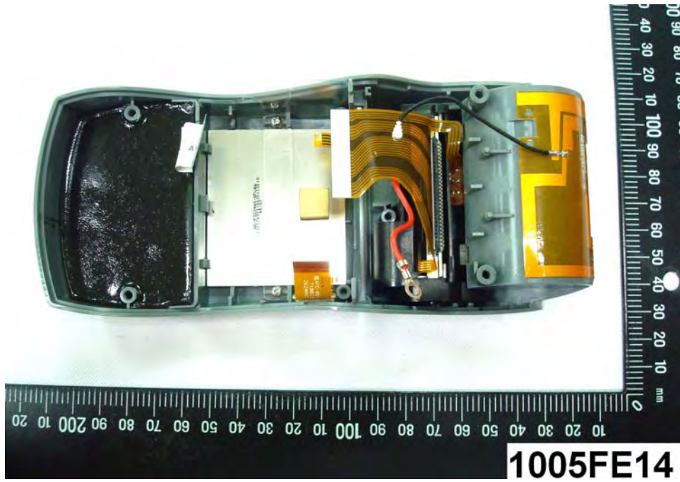
(29) EUT Photo
